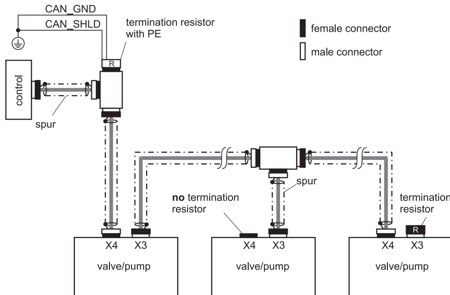
Figure 34: CAN wiring diagram
