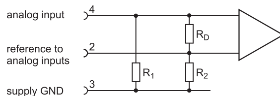
Figure 13: Equivalent circuit diagram of analog input
