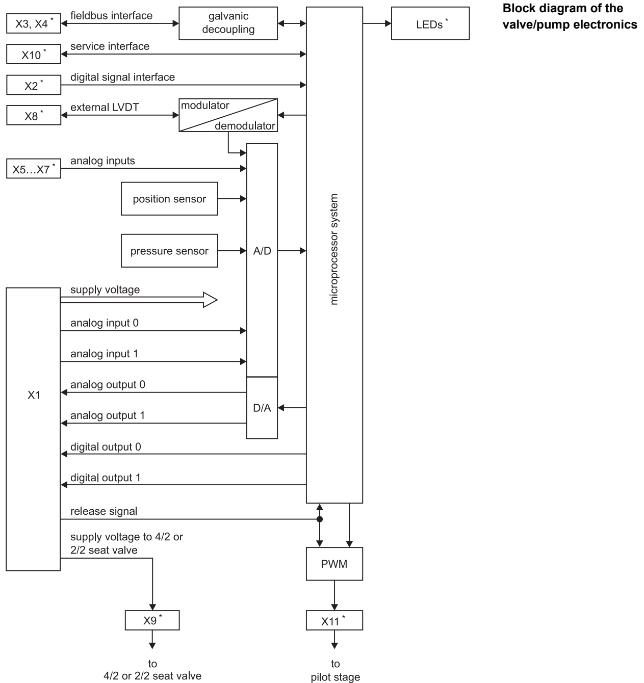
Figure 1: Block diagram of the valve/pump electronics
