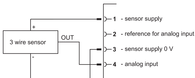
Figure 41: Connecting a 3-wire transducer to analog input connectors X5, X6 or X7
