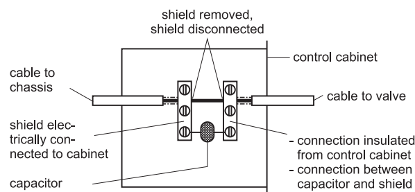
Figure 23: Connecting the insulated shielding to the control cabinet's wall (detail A from Figure 20)
