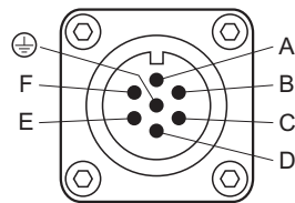
View of connector X1 (external thread, pin contacts)
