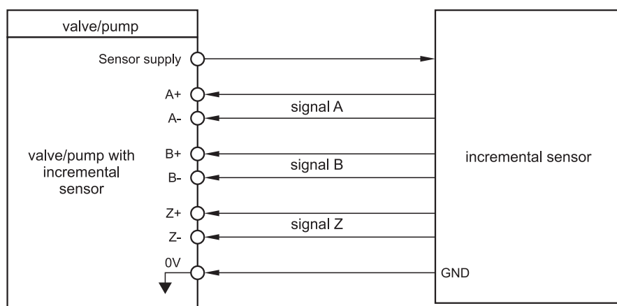
Figure 30: Wiring diagram with incremental transducer
