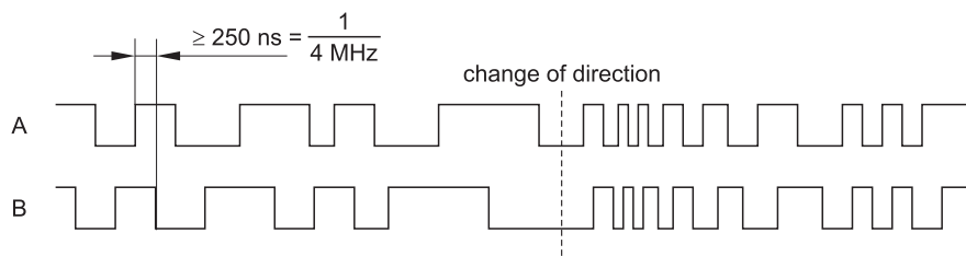
Figure 31: Incremental transducer signals A and B with reversal point and speed variation
