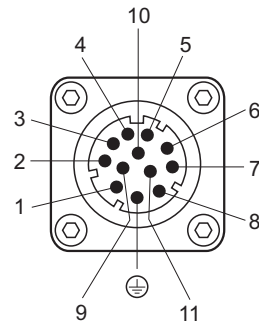
View of connector X1 (external thread, pin contacts)
