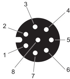
View of SSI transducer connector X2 (internal thread, socket connectors)
