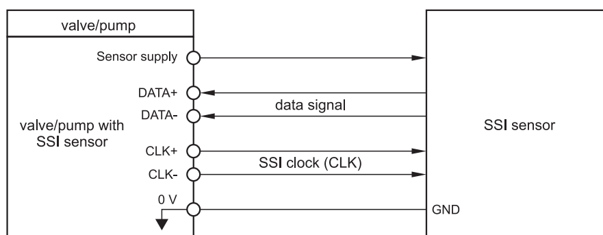
Figure 32: Wiring diagram with SSI transducer
