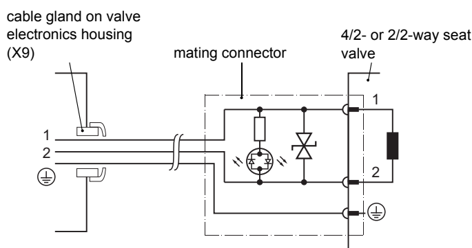
Figure 15: Block diagram of the plug connection of the 4/2- or 2/2-way seat valve (with free-wheeling and light emitting diode)
