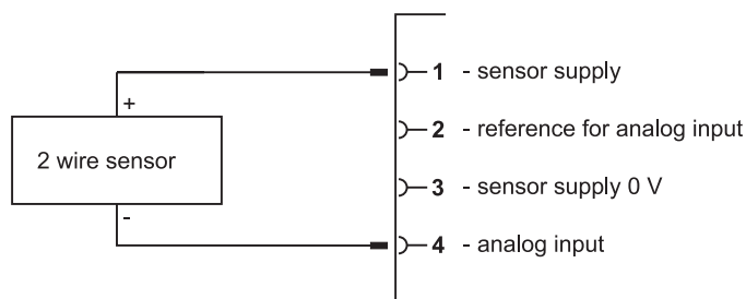
Figure 40: Connecting a 2-wire transducer to analog input connectors X5, X6 or X7
