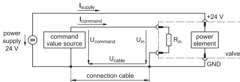
Figure 27: Circuit for single-ended command signals
