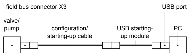
Figure 35: Connection of valve/pump to a PC via the CAN bus interface (connector X3)
