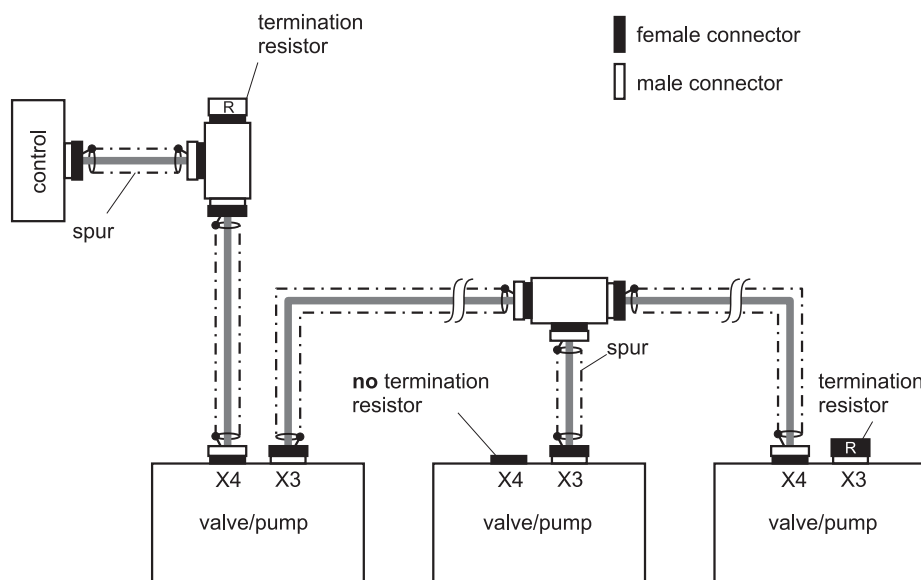
Figure 37: Profibus-DP wiring diagram
