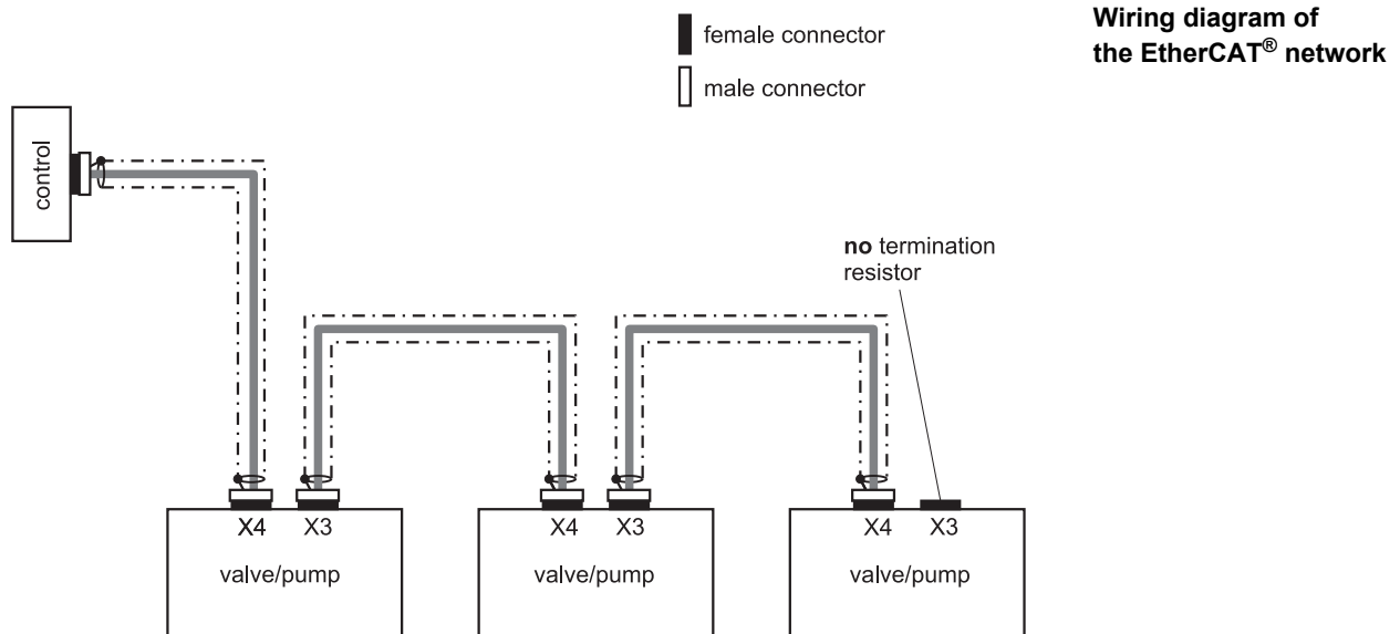
Figure 38: EtherCAT® wiring diagram
