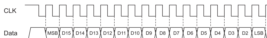
Figure 33: Signals between valve/pump and a 16-bit SSI transducer (example)
