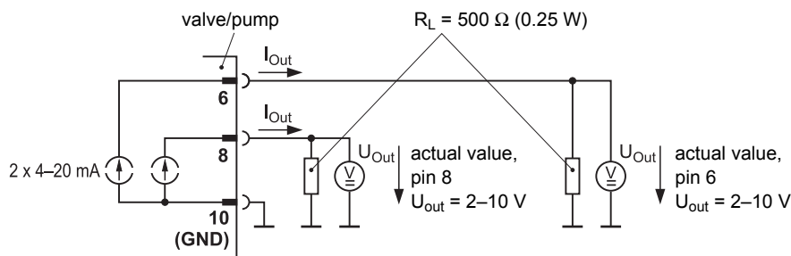
Figure 29: Circuit for converting the actual value output signals I_{out} (for valves with 11+PE-pin connector X1)
