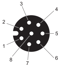
View of incremental transducer connector X2 (internal thread, socket connectors)
