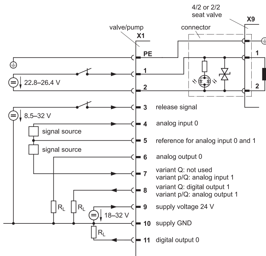
Figure 26: Wiring the 11+PE-pin connector X1
