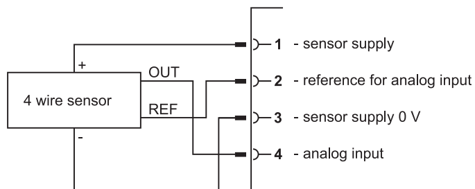
Figure 42: Connecting a 4-wire transducer to analog input connectors X5, X6 or X7
