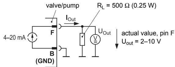
Figure 28: Circuit for converting the actual value output signals I_{out} (for valves with 6+PE-pin connector X1)
