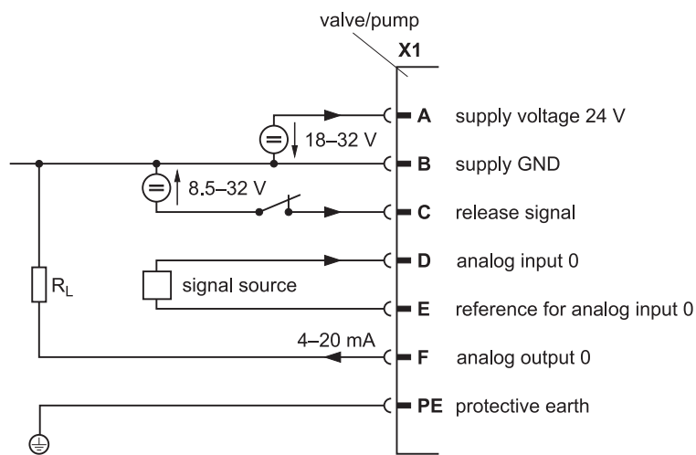
Figure 25: Wiring the 6+PE-pin connector X1
