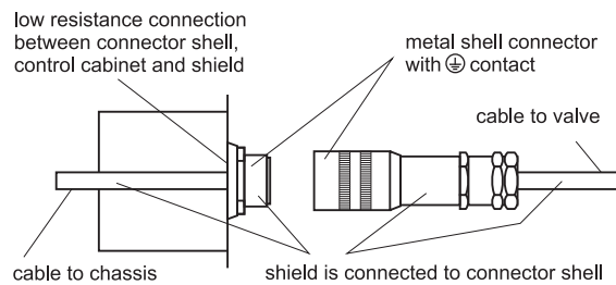
Figure 22: Connecting the cable shield via connector to the control cabinet's wall (detail A from Figure 20)
