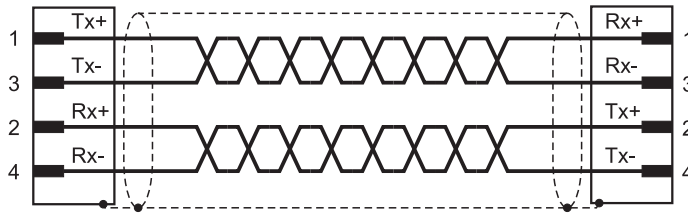
Figure 39: Twisted-pair wires in Ethernet/EtherCAT® cables with M12 connectors
