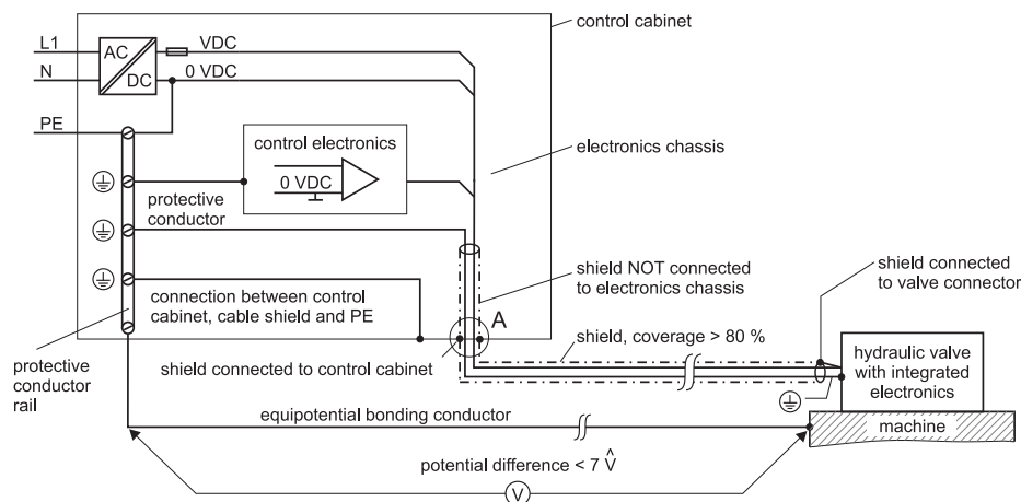
Figure 20: Equipotential bonding and protective grounding of machines (see also DIN EN 60204-1 ) and electrical shielding of our valves/pumps with integrated electronics
