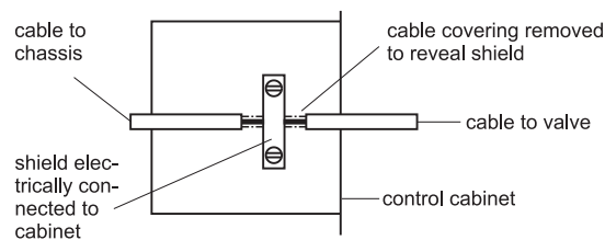
Figure 21: Connecting the shield to the control cabinet's wall (detail A from Figure 20)
