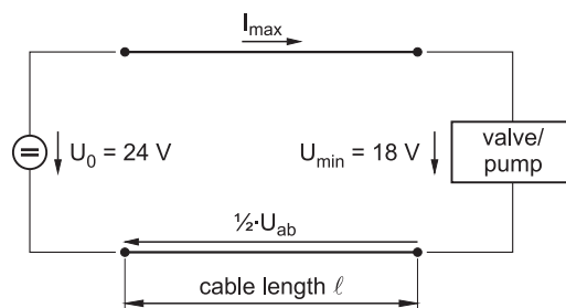
Figure 24: Voltage drop on the supply cable
