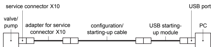
Figure 36: Connection of valve/pump to a PC via the service interface (service connector X10)
