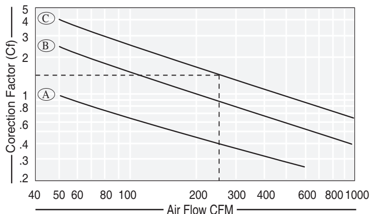
Air Flow Correction Chart
