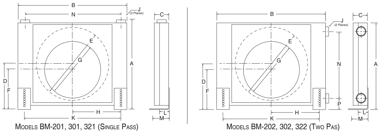
STANDARD DIMENSIONS (inches)
