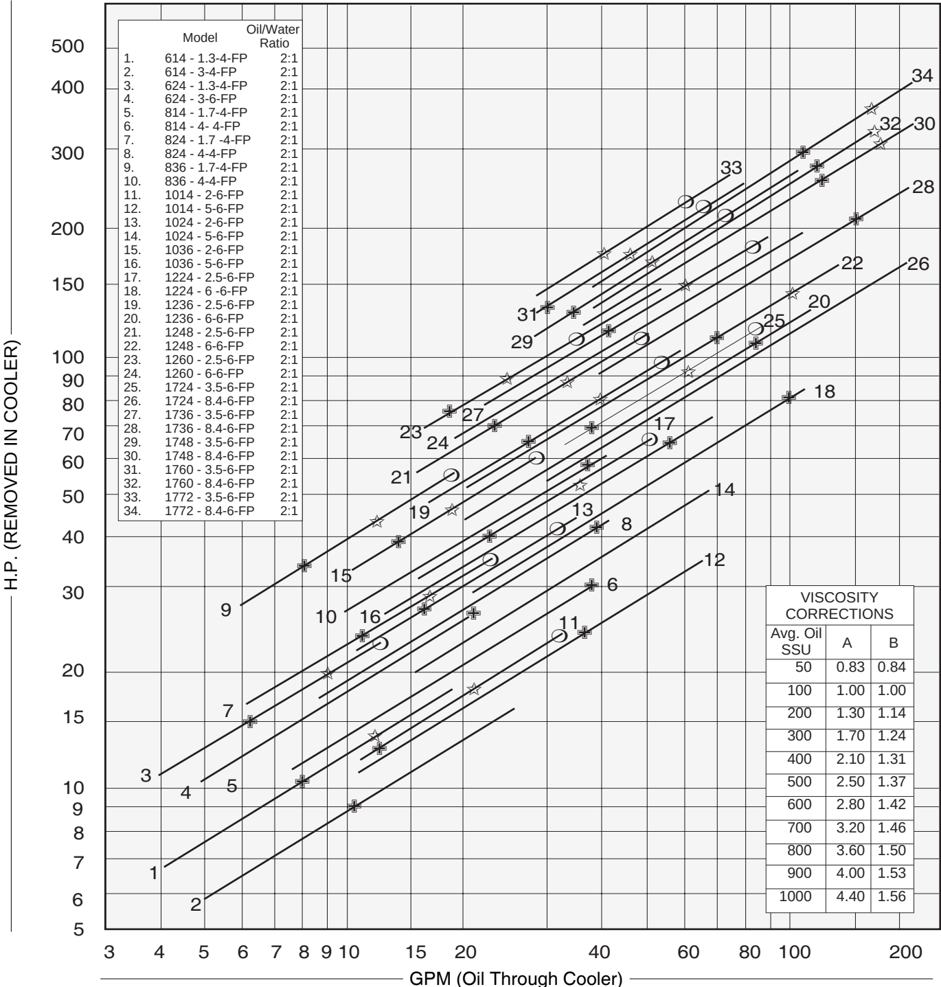
HEAT ENERGY DISSIPATION RATES (Basic Stock Model)
