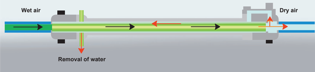
Working principle of membrane dryers.
