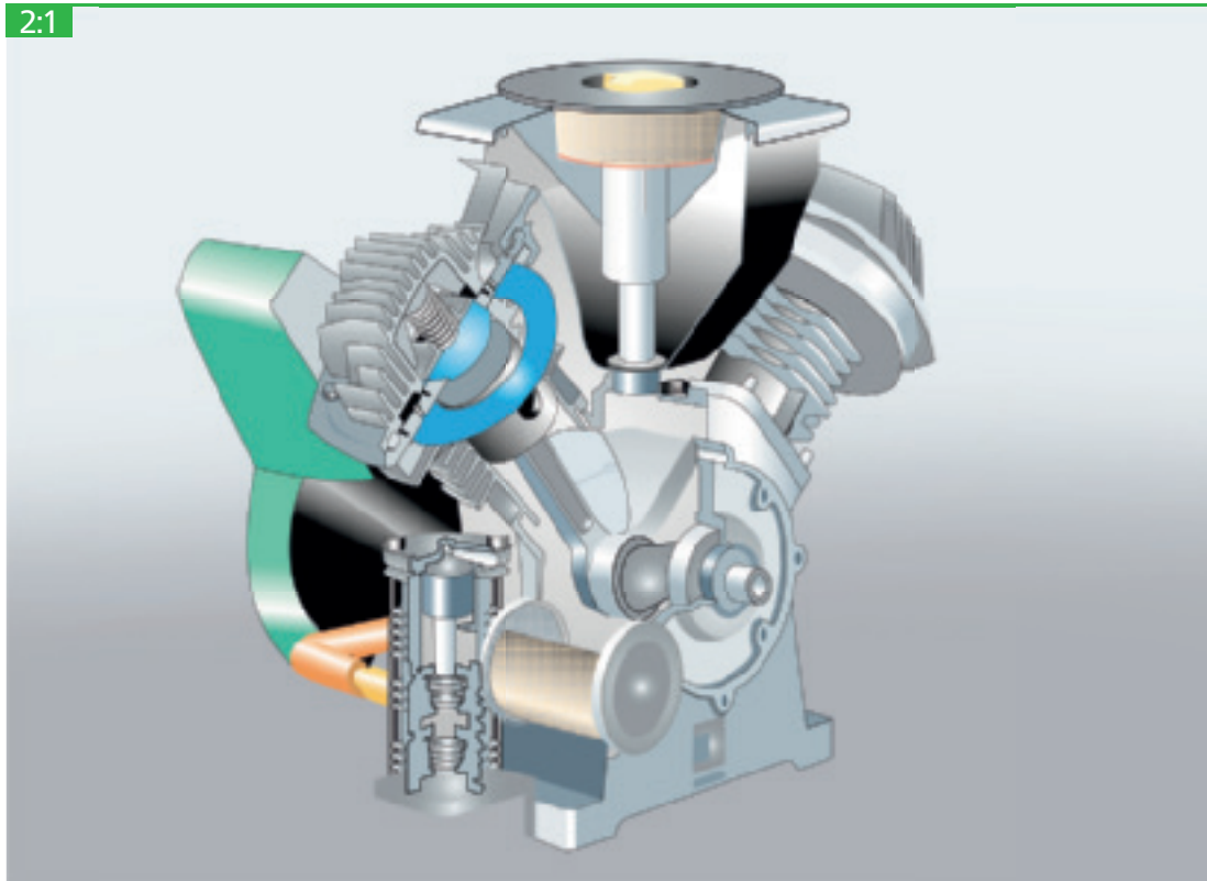
Piston compressor.
