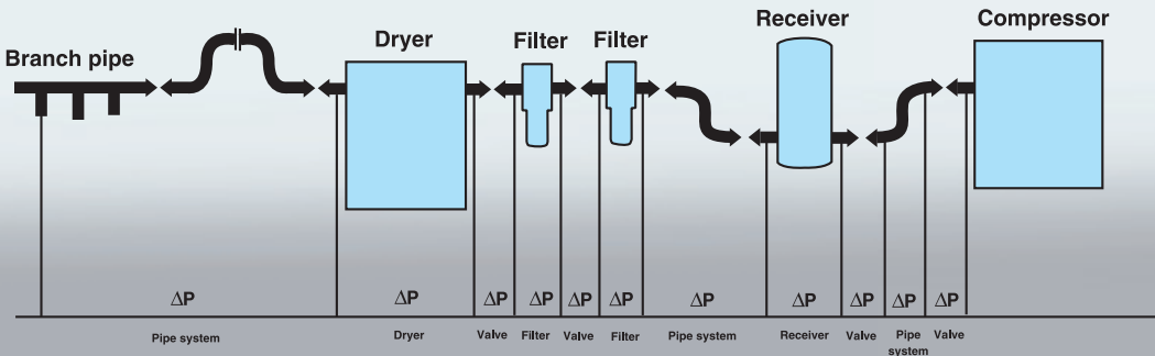
The pressure drop across different components in the network affects the requisite working pressure.
