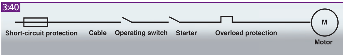
Simplified schematic for electric motor connection to mains power supply.
