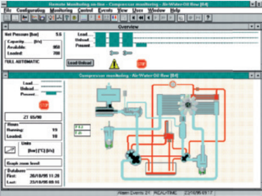
An overview display with remote monitoring. The upper section shows the installation status. Three machines in operation, one stopped. In the lower section details for compressor 4 are shown, among others, flow chart for the compressed air, cooling water and oil as well as prevailing compressor data.
