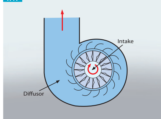
Radial turbocompressor.
