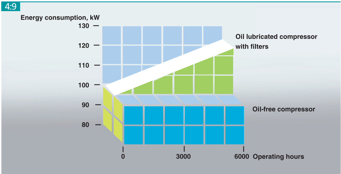
Oil-free compressors give constant compressed air quality at a fixed energy cost.
