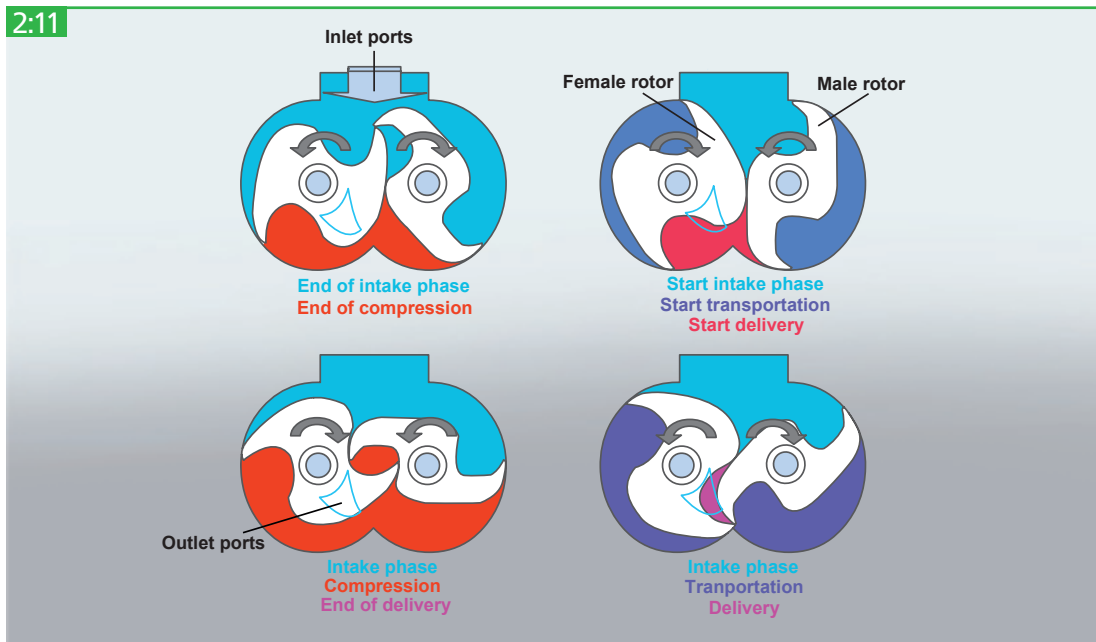
Compression principle of the double tooth compressor.
