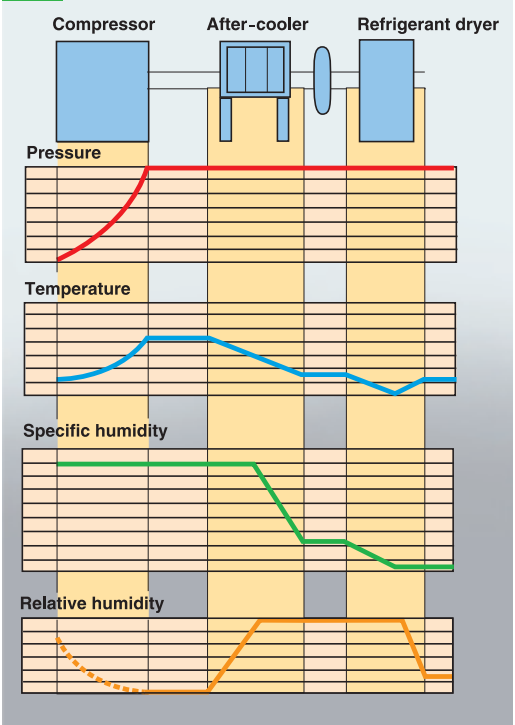
Typical parameter changes with compression, after-cooling and refrigerant drying.
