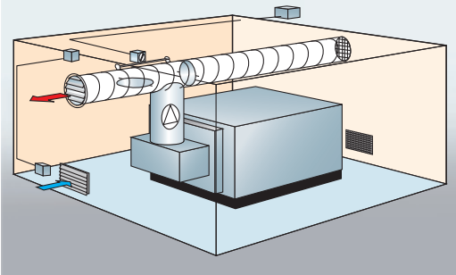
Energy recovery from an air-cooled compressor.
