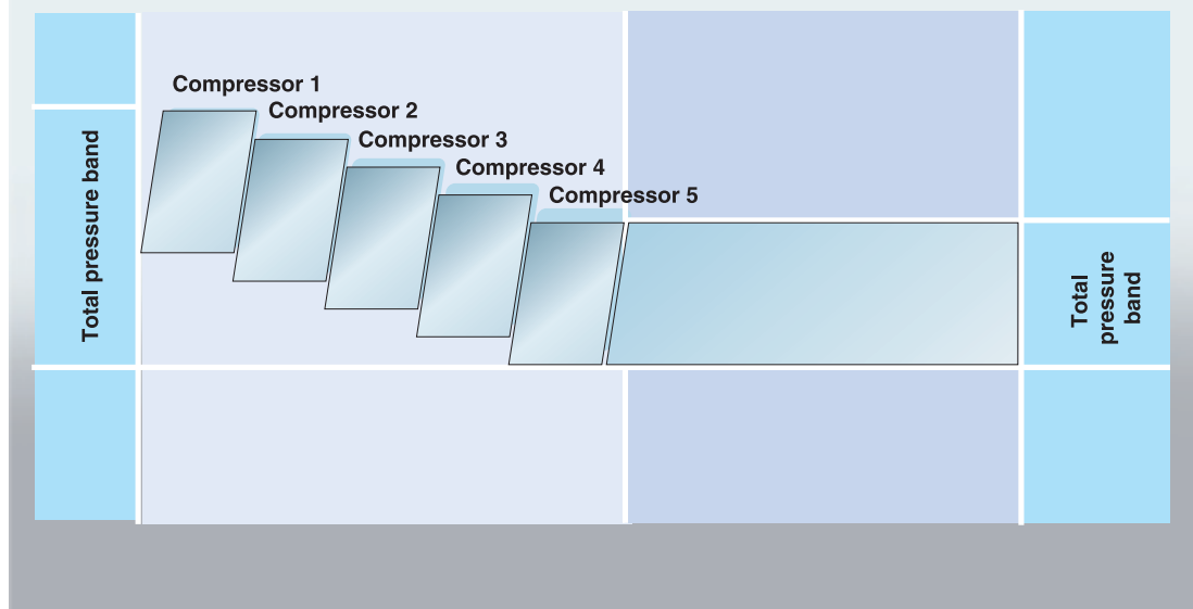
Illustration of the pressure band for five compressors controlled by conventional pressure switches (left-hand field) and the same machines controlled by a regulation system (right-hand field).
