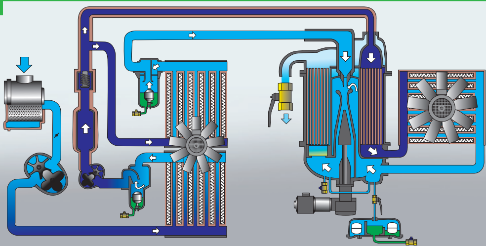
Heat of Compression (HOC) type dryer – MD model with rotating drum.
