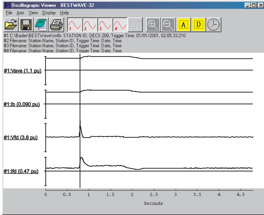
Figure 6 - BESTwave Oscillography
