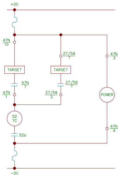
CONTROL CIRCUIT
