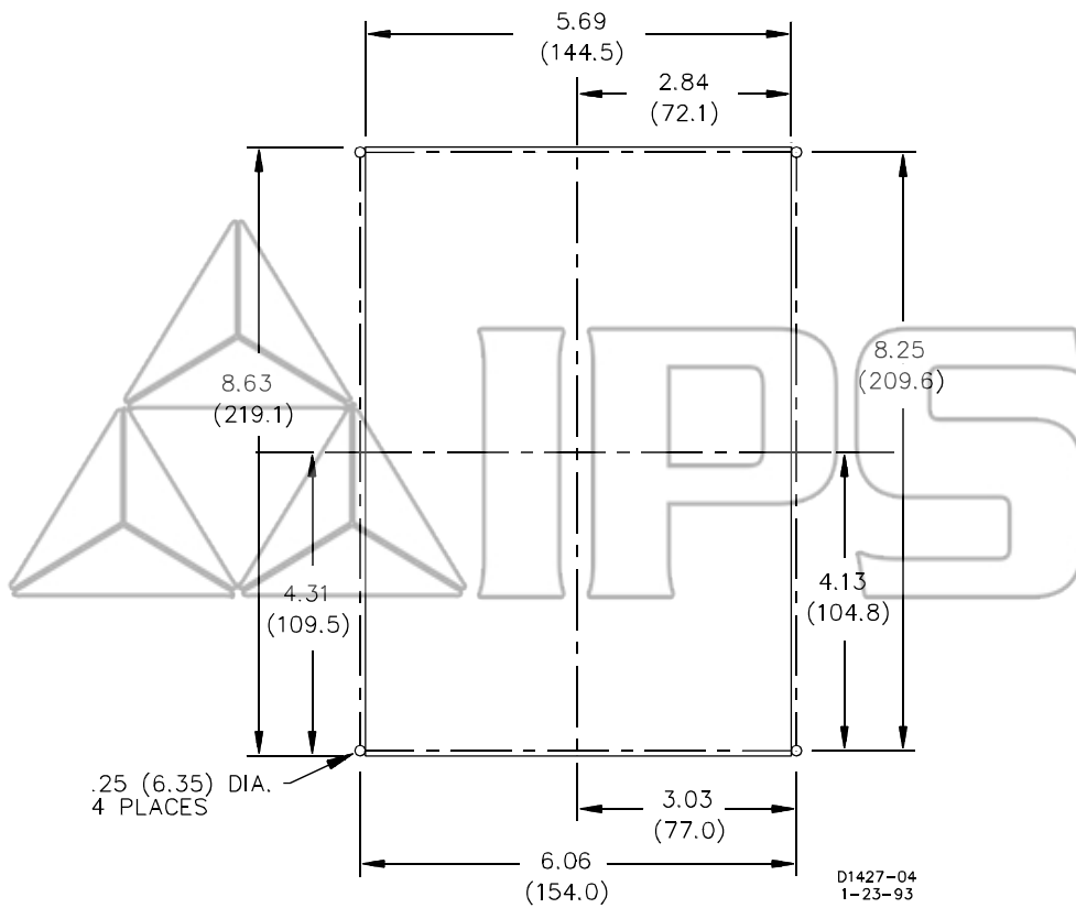
Figure 4-1. S1 Case, Panel Drilling Diagram, Semi-Flush Mounting
