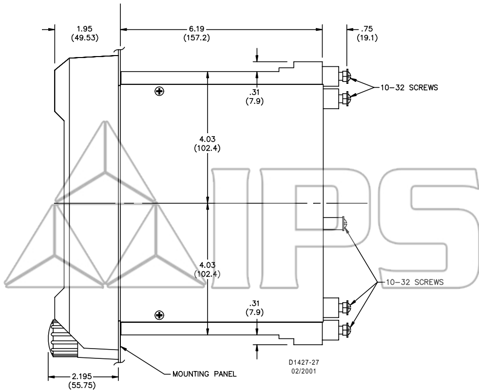
Figure 4-5. S1 Case, Double-Ended, Semi-Flush Mounting, Outline Dimensions, Side View
