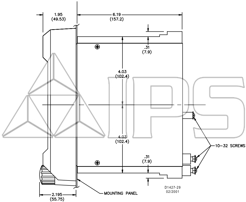
Figure 4-3. S1 Case, Single-Ended, Semi-Flush Mounting, Outline Dimensions, Side View
