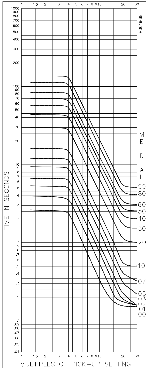
Figure A-67. Timing Type C7, I_t Limit #7 with Integrated Algorithm and Extended Timing
