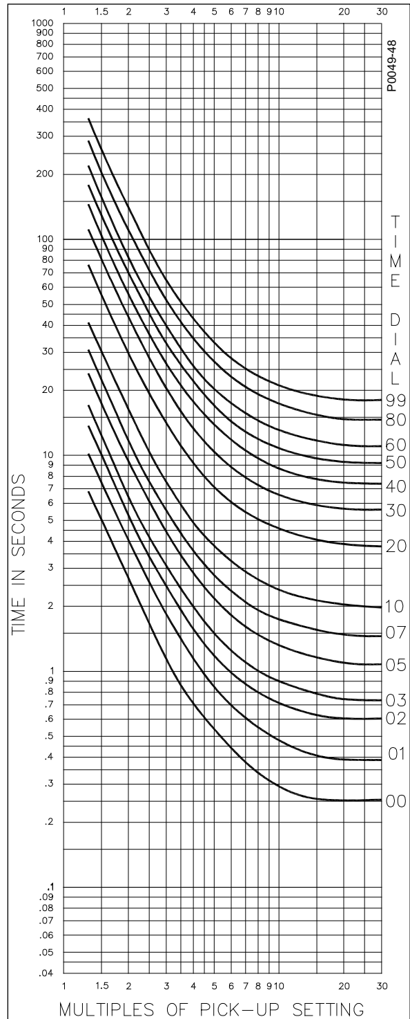
Figure A-47. Timing Type B5, Inverse with Integrated Algorithm and Extended Timing
