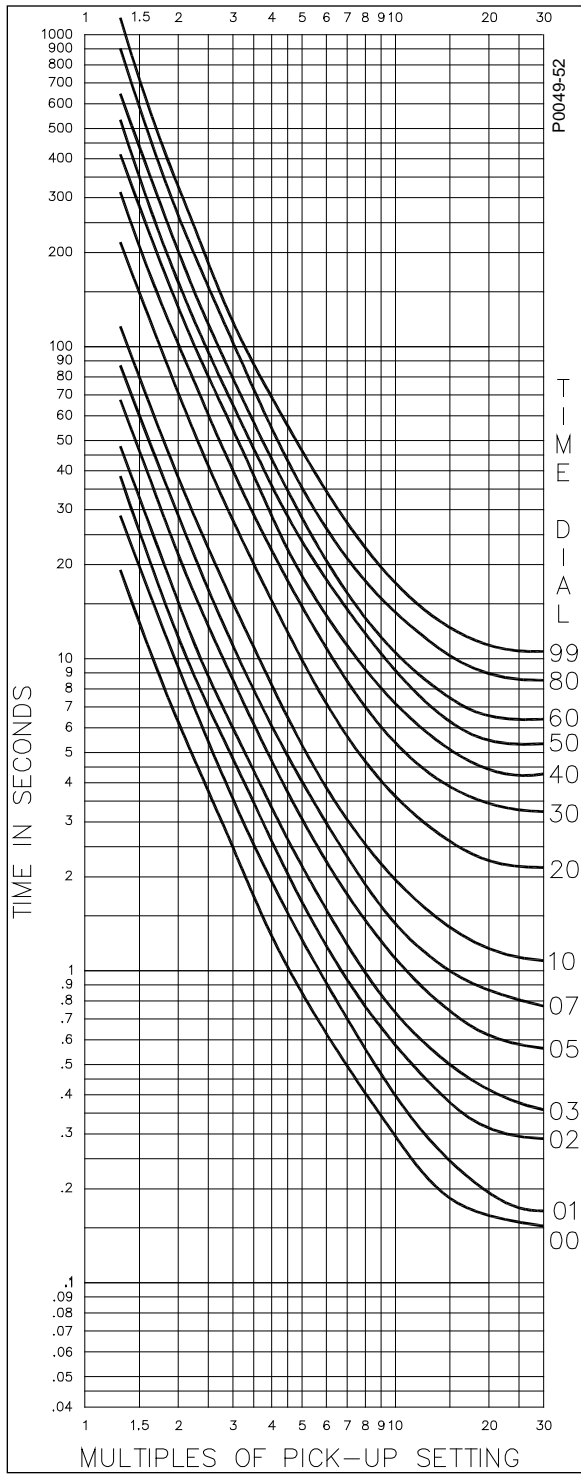
Figure A-51. Timing Type B7, Extremely Inverse with Integrated Algorithm and Extended Timing
