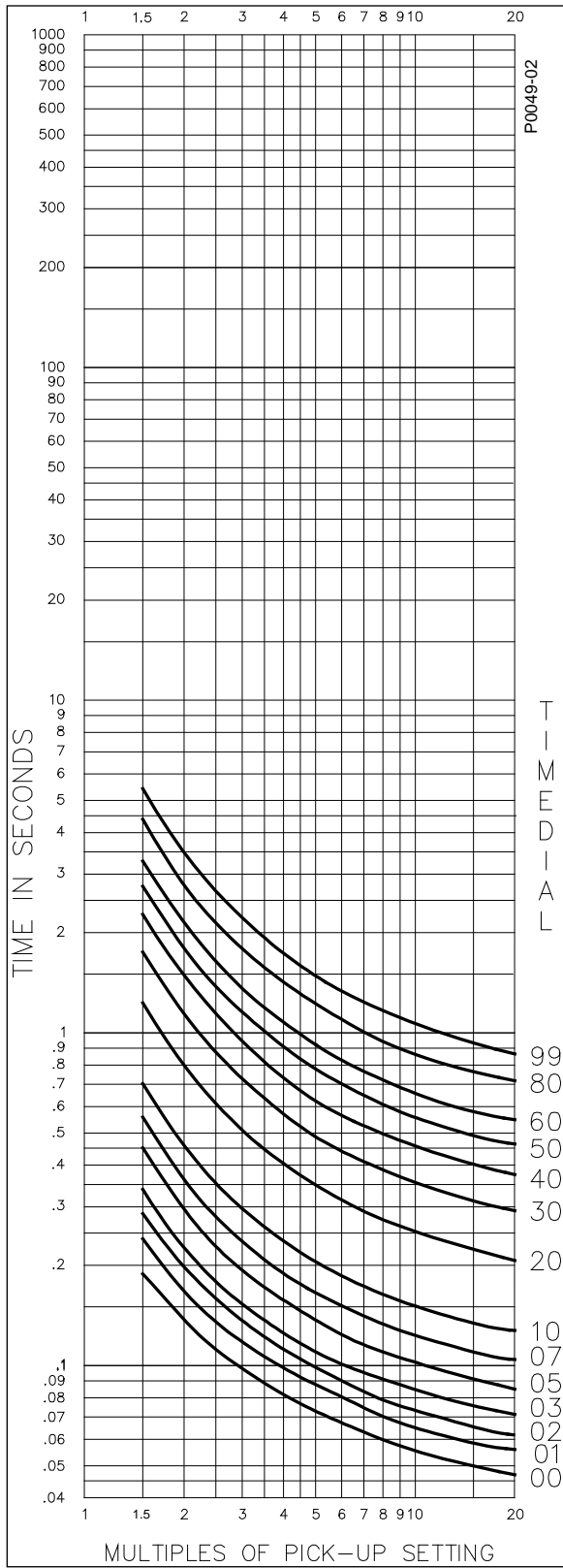
Figure A-1. Timing Type B1, Short Inverse
