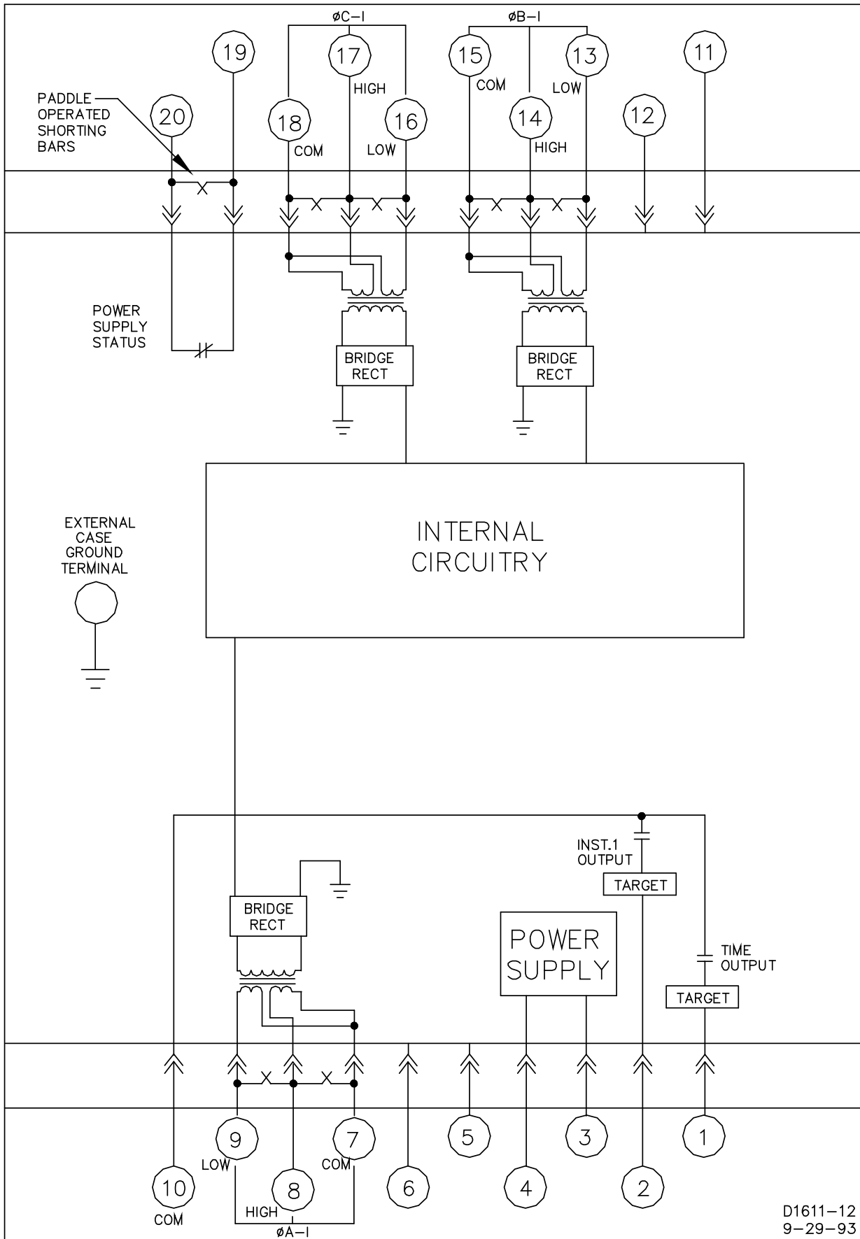
Figure 4-12. Typical Internal Diagram, Sensing Input Type G
