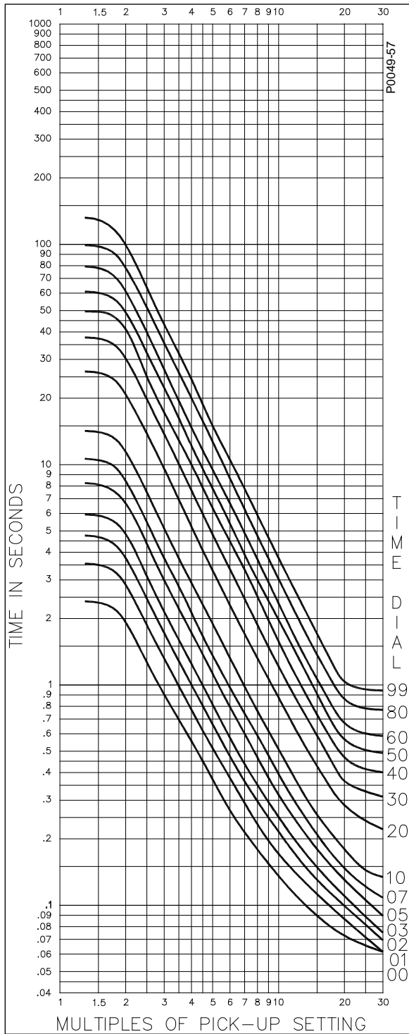
Figure A-56. Timing Type C2, I^2t Limit #2 with Integrated Algorithm
