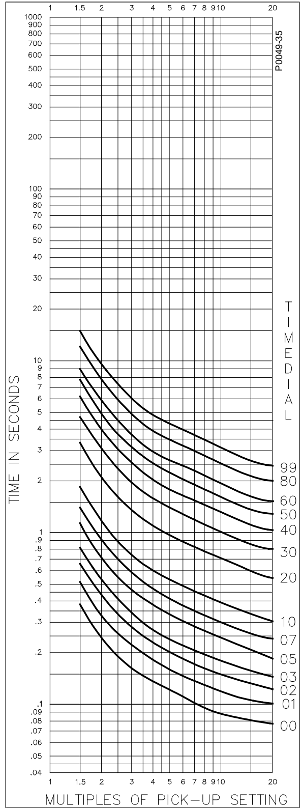
Figure A-34. Timing Type E4, BS 142 Inverse
