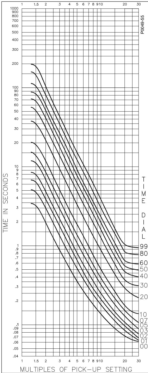
Figure A-54. Timing Type C1, I^2t Limit #1 with Integrated Algorithm
