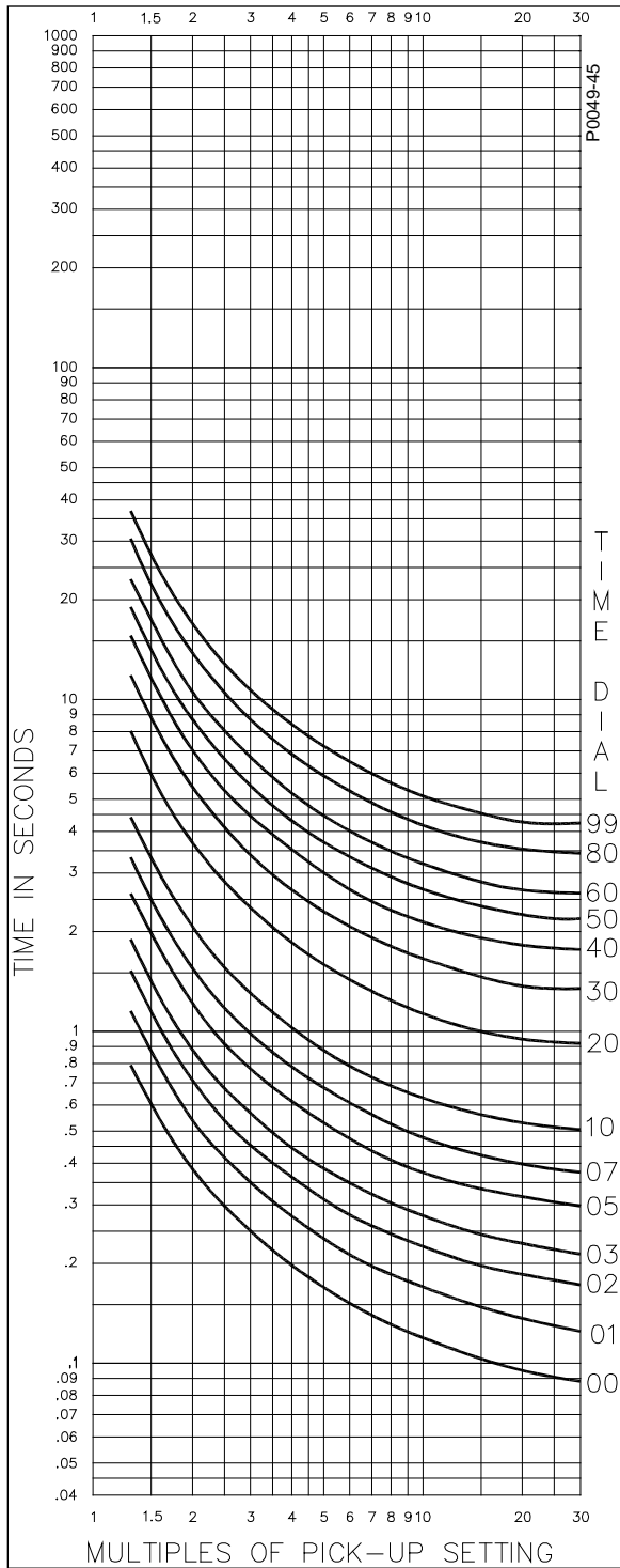
Figure A-44. Timing Type B4, Moderately Inverse with Integrated Algorithm.
