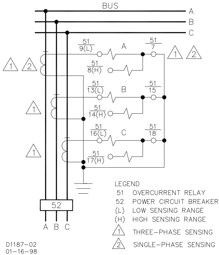
Figure 4-7. Typical Sensing External Connections, Sensing Input Type G or K
