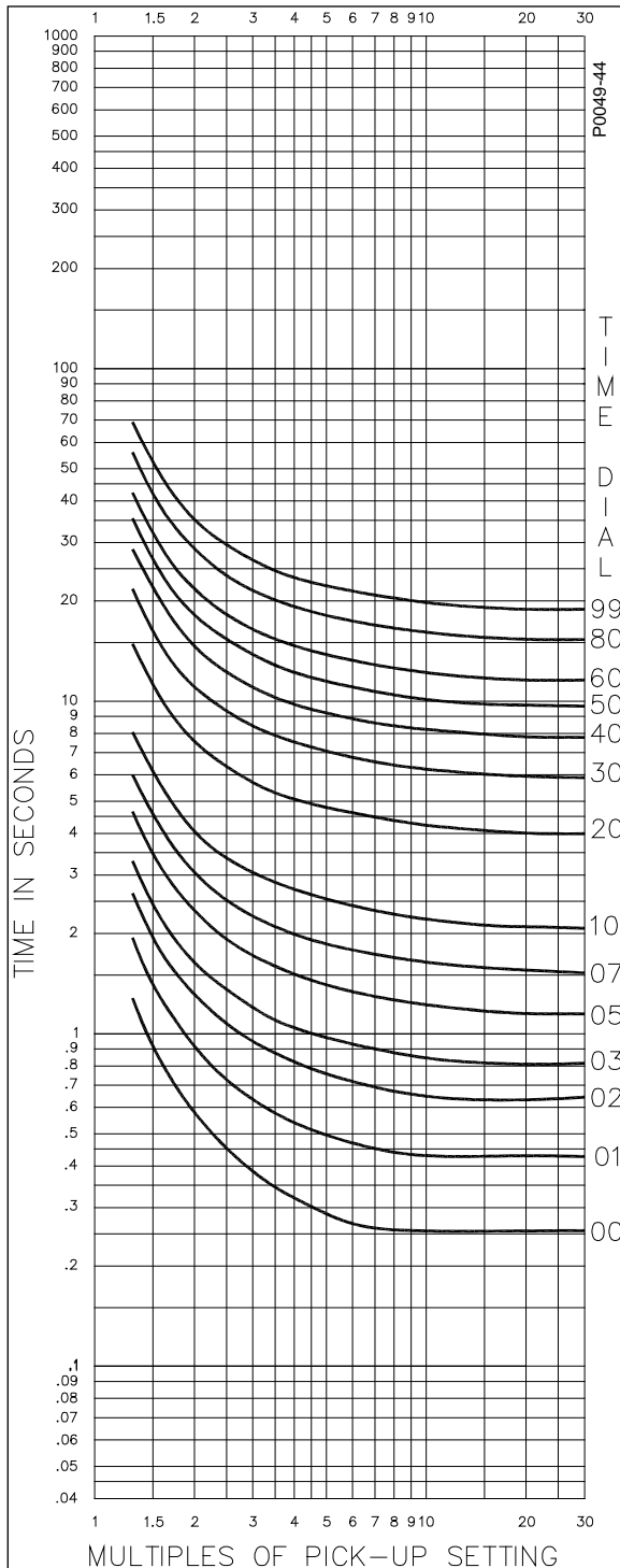
Figure A-43. Timing Type B3, Definite Time with Integrated Algorithm and Extended Timing
