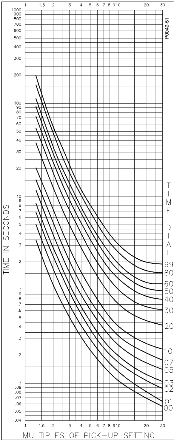
Figure A-50. Timing Type B7, Extremely Inverse with Integrated Algorithm
