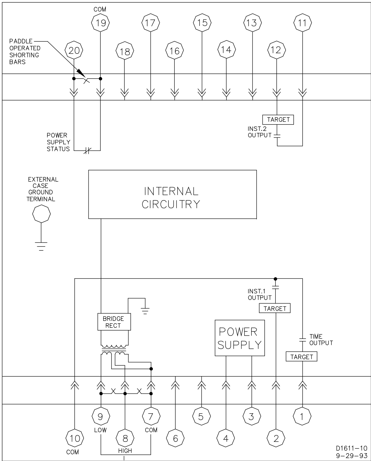
Figure 4-10. Typical Internal Diagram, Sensing Input Type K
