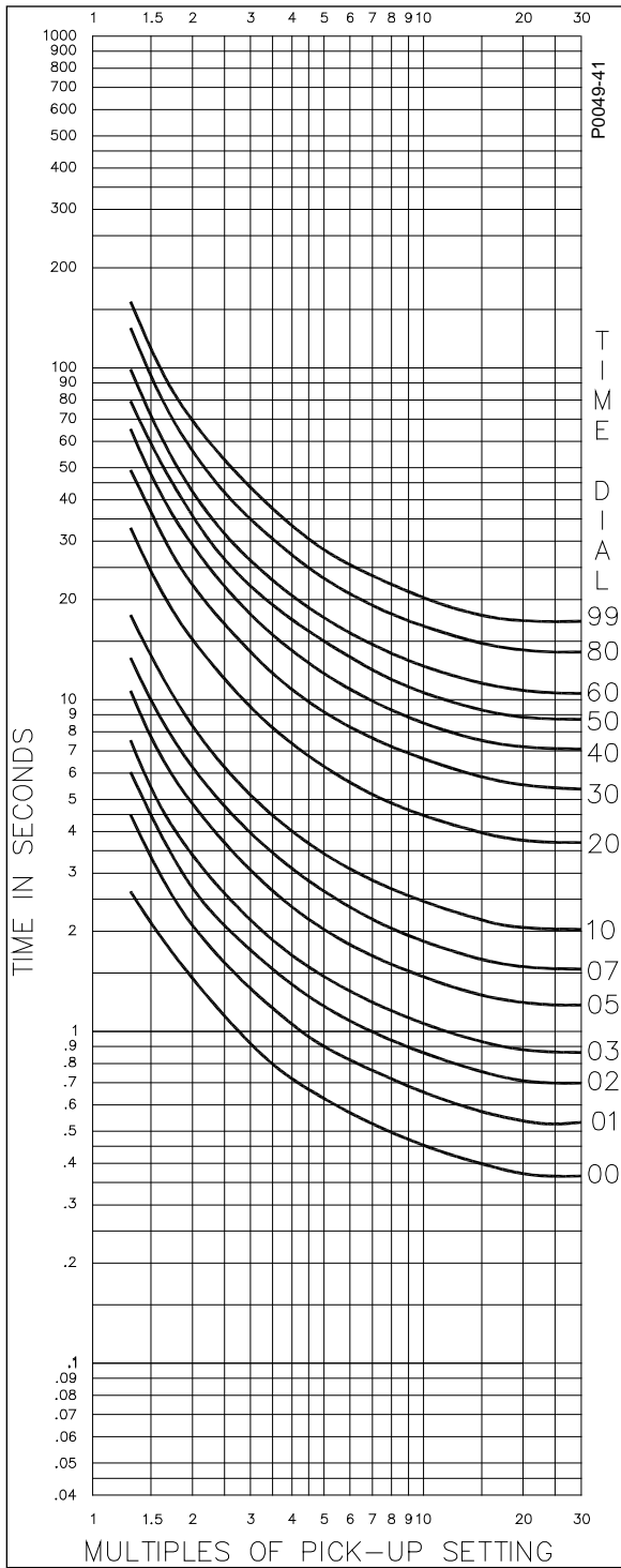
Figure A-40. Timing Type B2, Long Inverse with Integrated Algorithm
