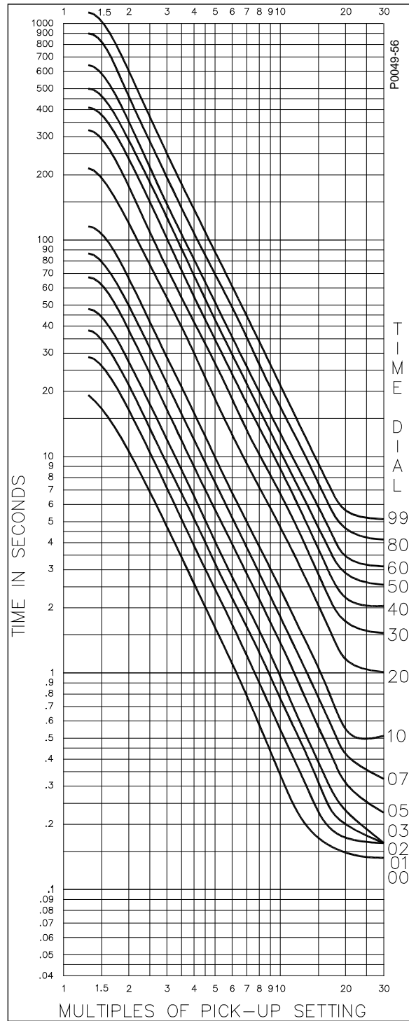
Figure A-55. Timing Type C1, I^2t Limit #1 with Integrated Algorithm
