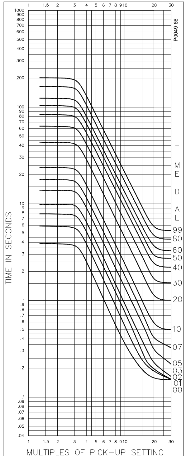
Figure A-65. Timing Type C6, f_t Limit #6 with Integrated Algorithm and Extended Timing
