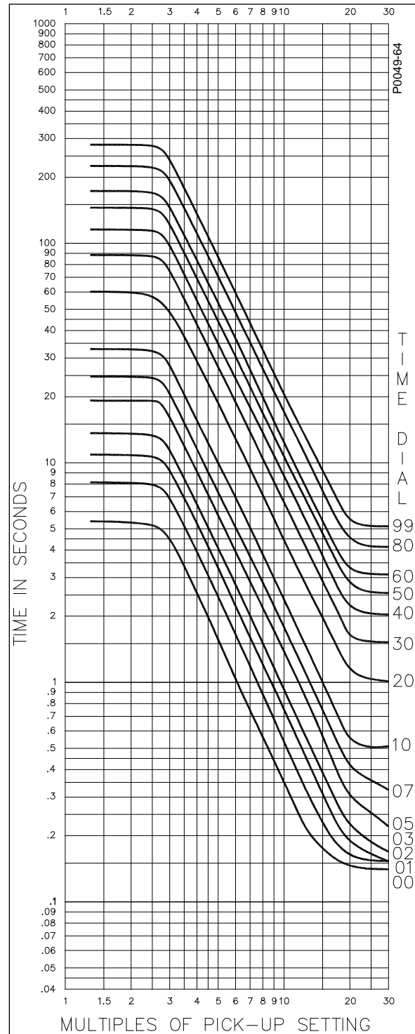
Figure A-63. Timing Type C5, I^2t Limit #5 with Integrated Algorithm and Extended Timing
