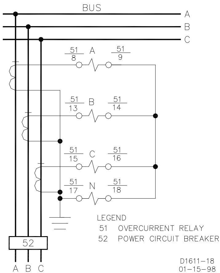
Figure 4-9. Typical Sensing External Connections, Sensing Input Type H or V
