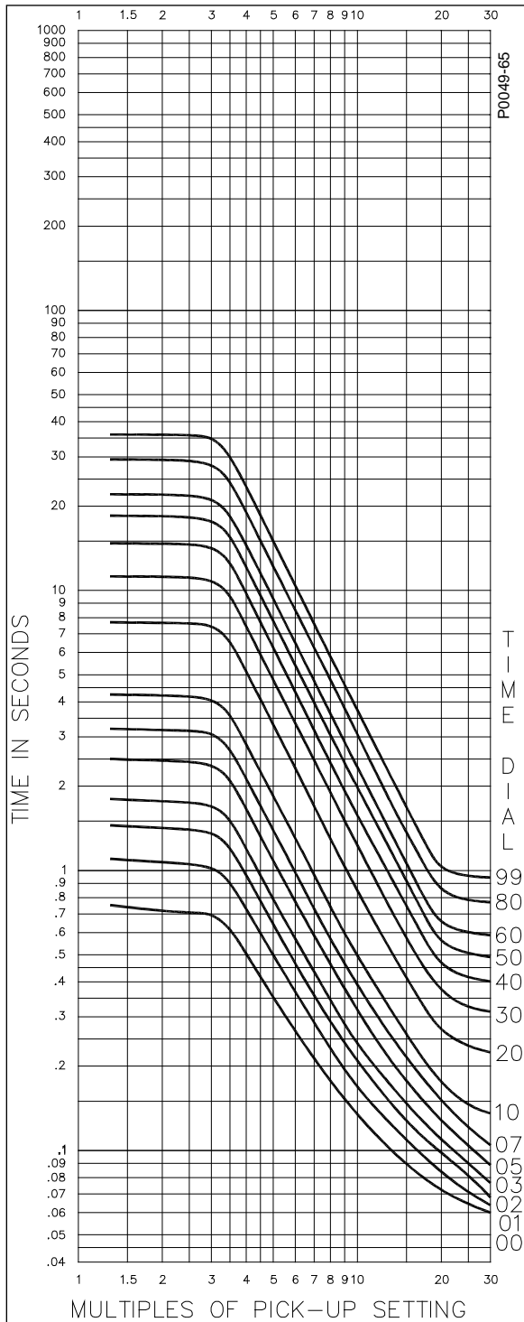
Figure A-64. Timing Type C6, f_t Limit #6 with Integrated Algorithm
