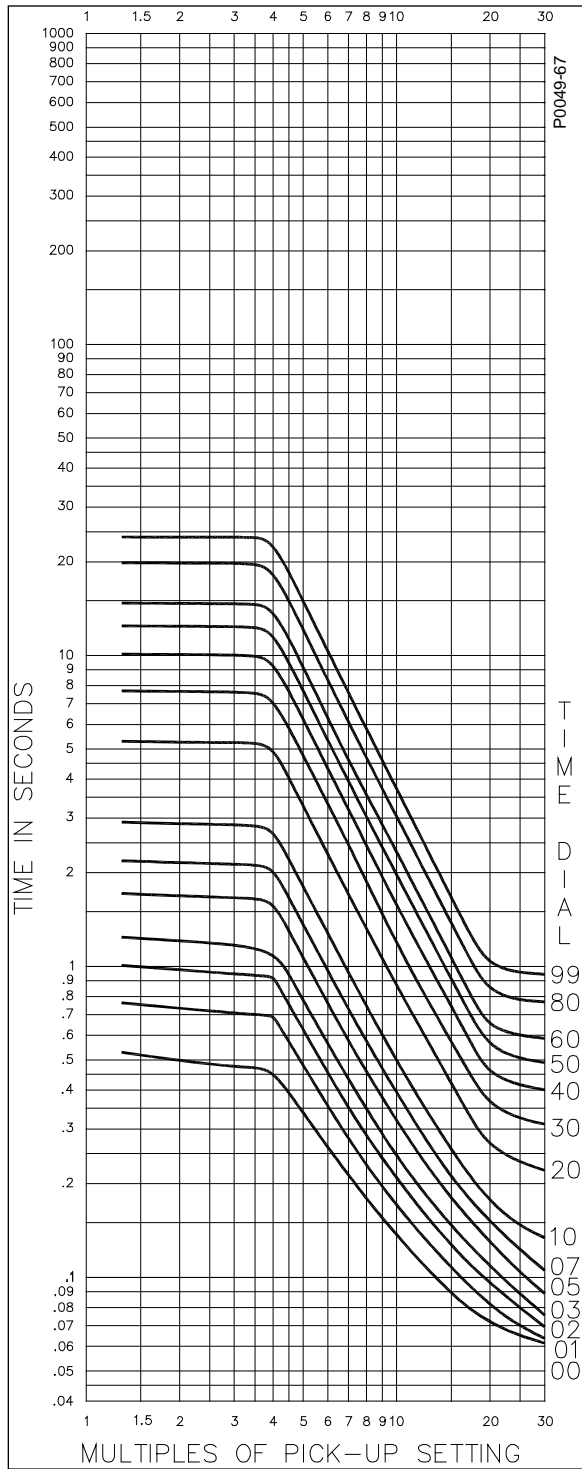
Figure A-66. Timing Type C7, I_t Limit #7 with Integrated Algorithm
