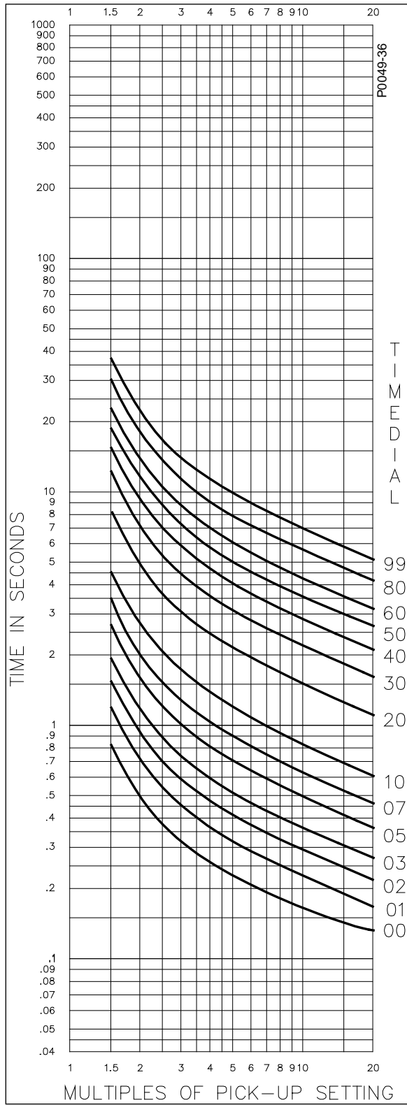
Figure A-35. Timing Type E5, BS 142 Inverse
