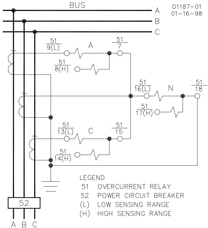
Figure 4-8. Typical Sensing External Connections, Sensing Input Type I or X
