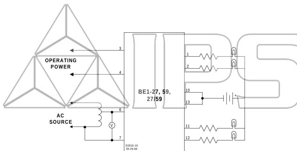
Figure 5-1. Pickup and Dropout Test Circuit Diagram
