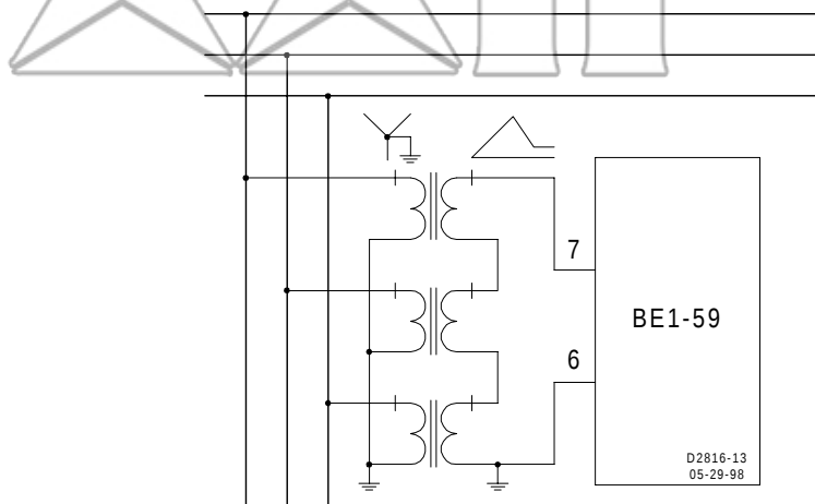
Figure 1-1. Ground Fault Detection
