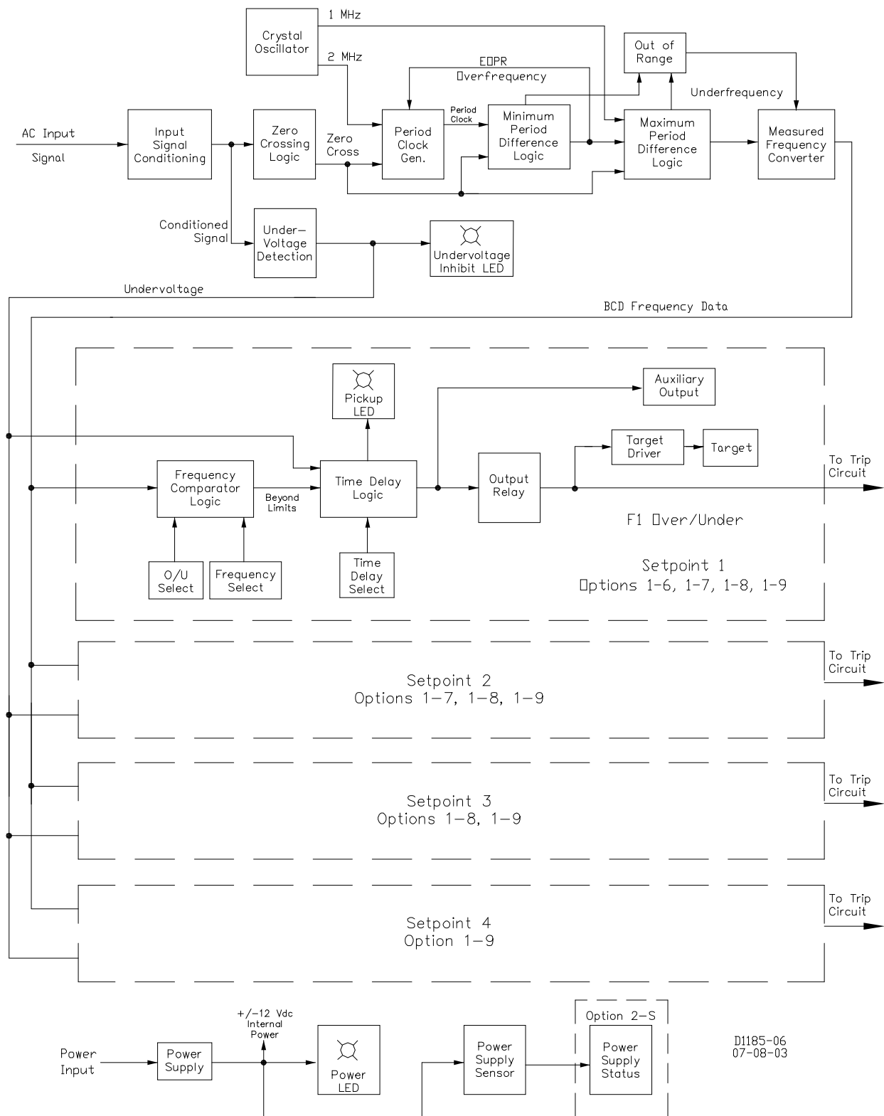
Figure 3-1. BE1-810/U Functional Block Diagram
