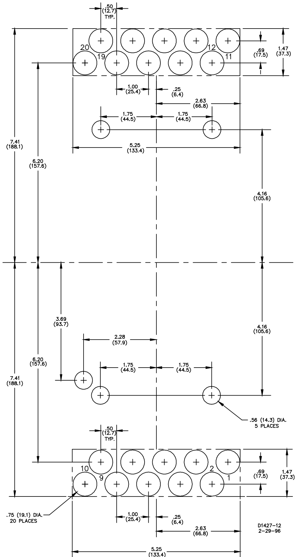
Figure 4-13. M1 Case, Panel Cutting/Drilling Diagram, Projection Mounting, Rear View
