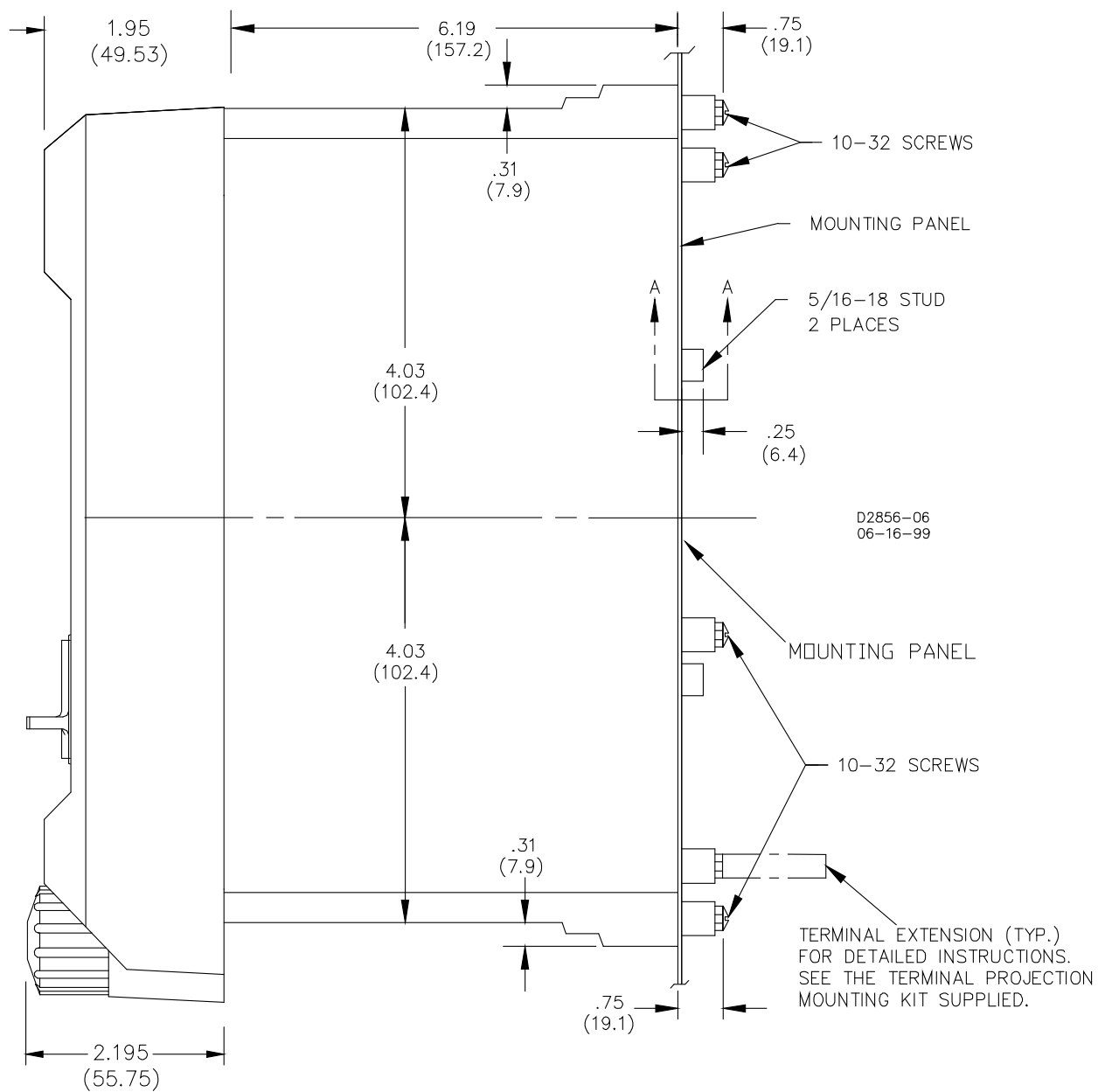
Figure 4-9. S1 Case Dimensions, Double-Ended, Projection Mounting, Side View
