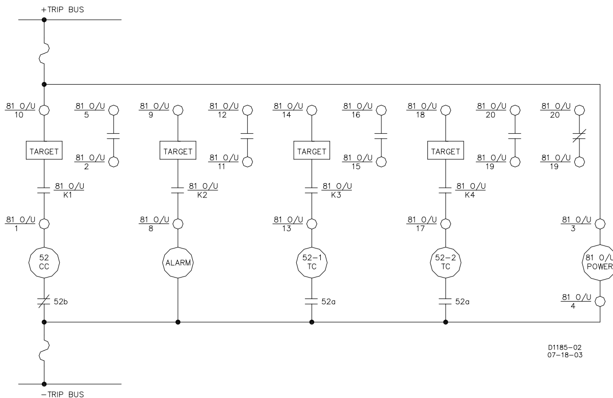
Figure 4-19. Typical DC Connections
