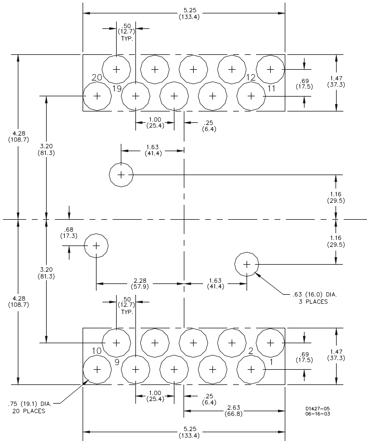
Figure 4-2. S1 Case, Panel Cutting/Drilling Diagram, Double-Ended, Projection Mounting, Rear View
