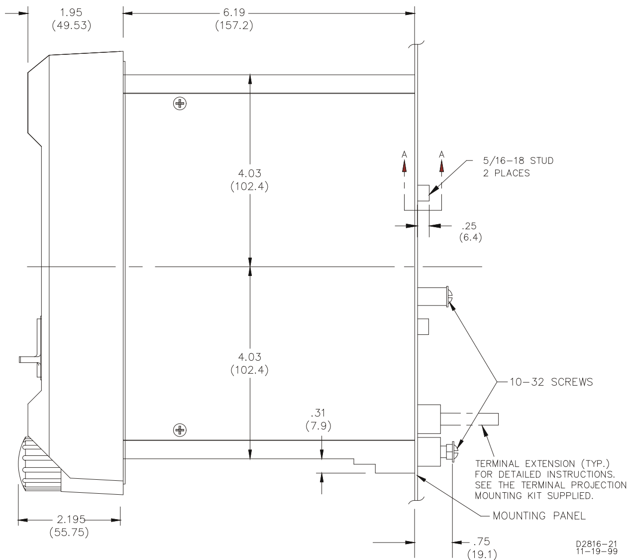
Figure 4-11. S1 Case Dimensions, Single-Ended, Projection Mounting, Side View
