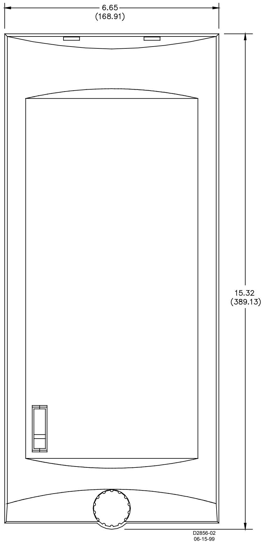
Figure 4-14. M1 Case (Cover) Dimensions, Front View
