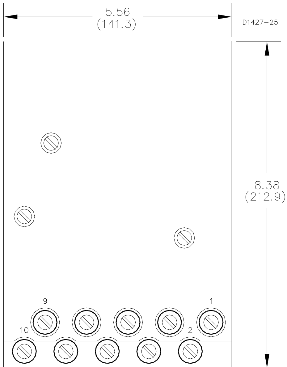
Figure 4-7. S1 Case Dimensions, Single-Ended, Projection Mounting, Rear View
