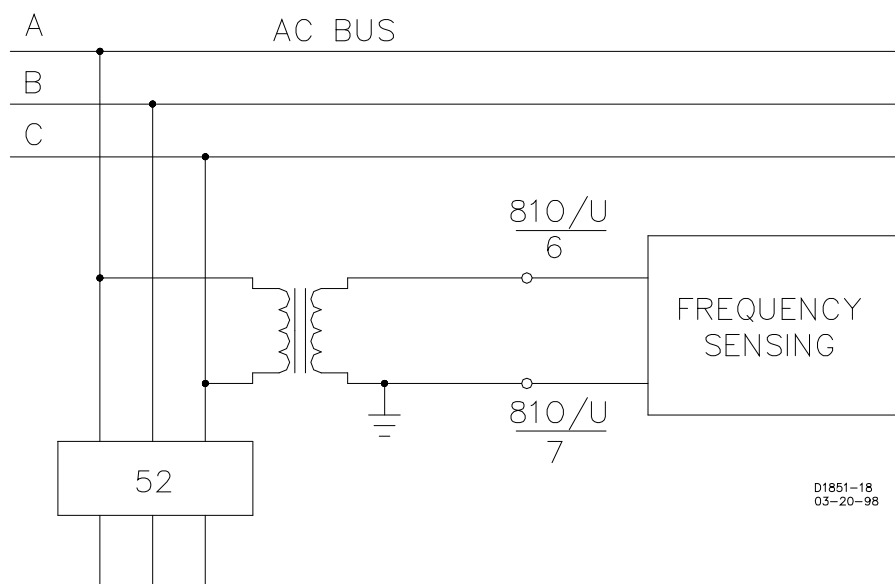
Figure 4-20. Typical AC Sensing Connections
