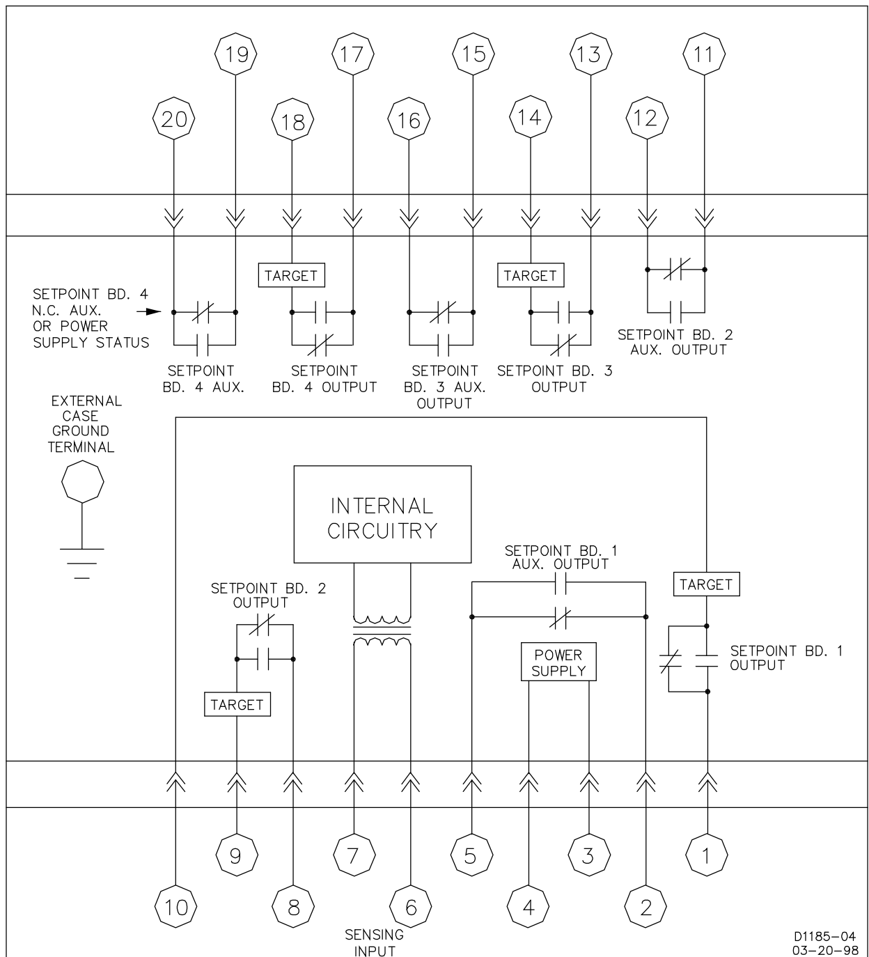
Figure 4-18. Internal Relay Connections
