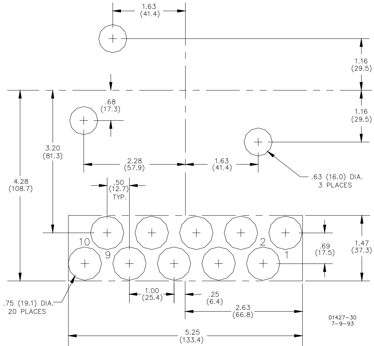
Figure 4-3. S1 Case, Panel Cutting/Drilling Diagram, Single-Ended, Projection Mounting, Rear View
