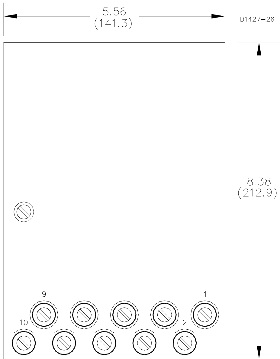
Figure 4-6. S1 Case Dimensions, Single-Ended, Semi-Flush Mounting, Rear View
