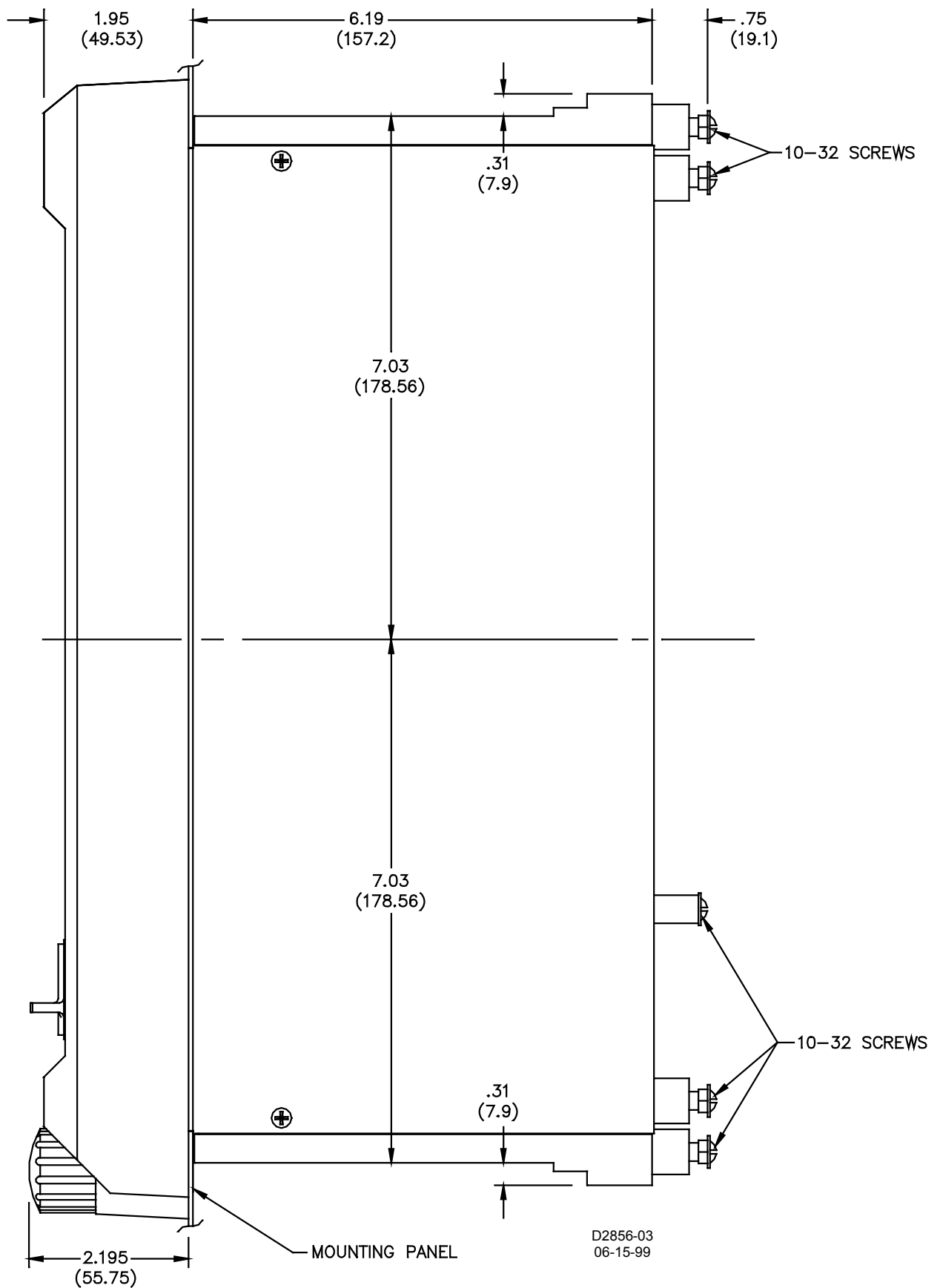
Figure 4-16. M1 Case Dimensions, Semi-Flush Mounting, Side View
