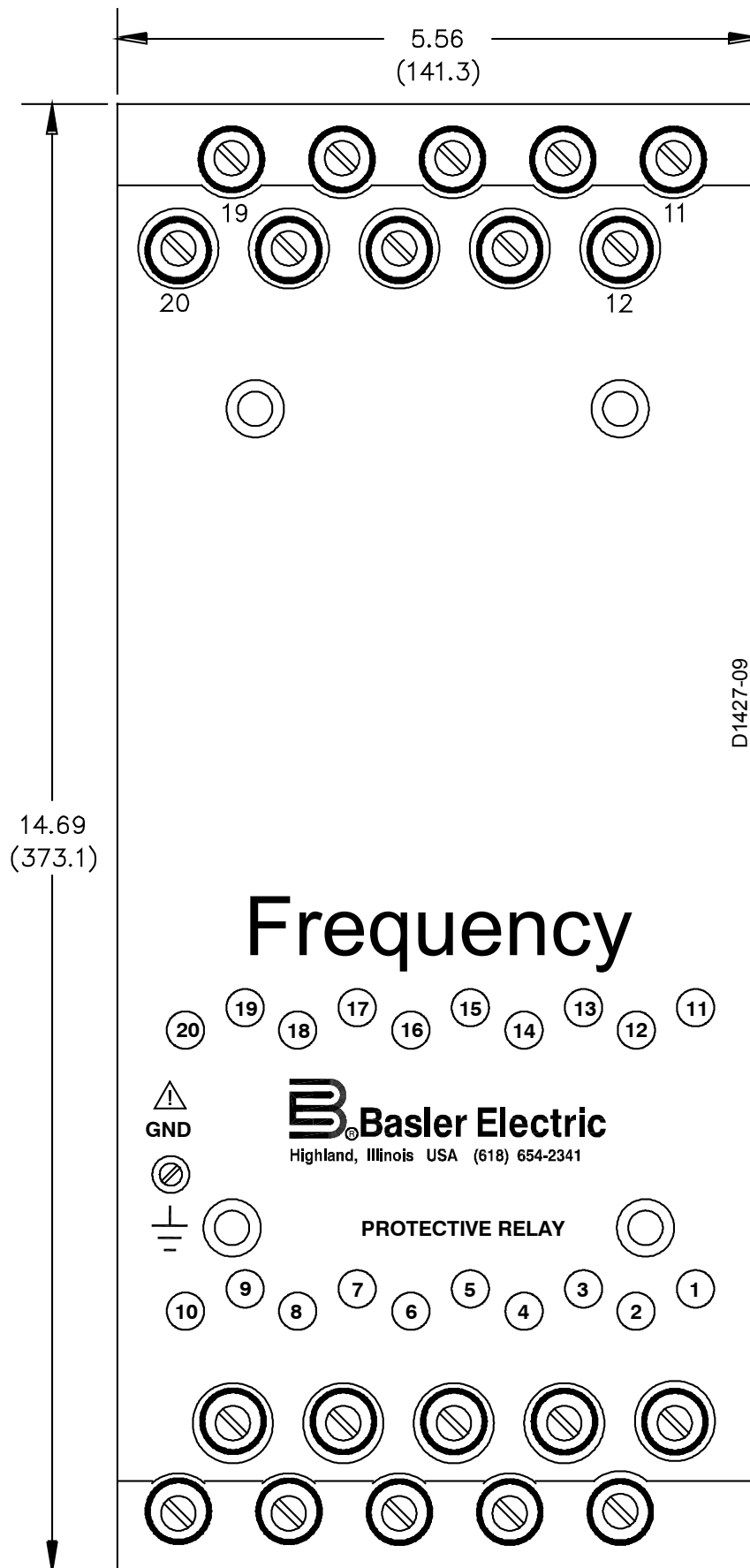
Figure 4-15. M1 Case Dimensions, Rear View
