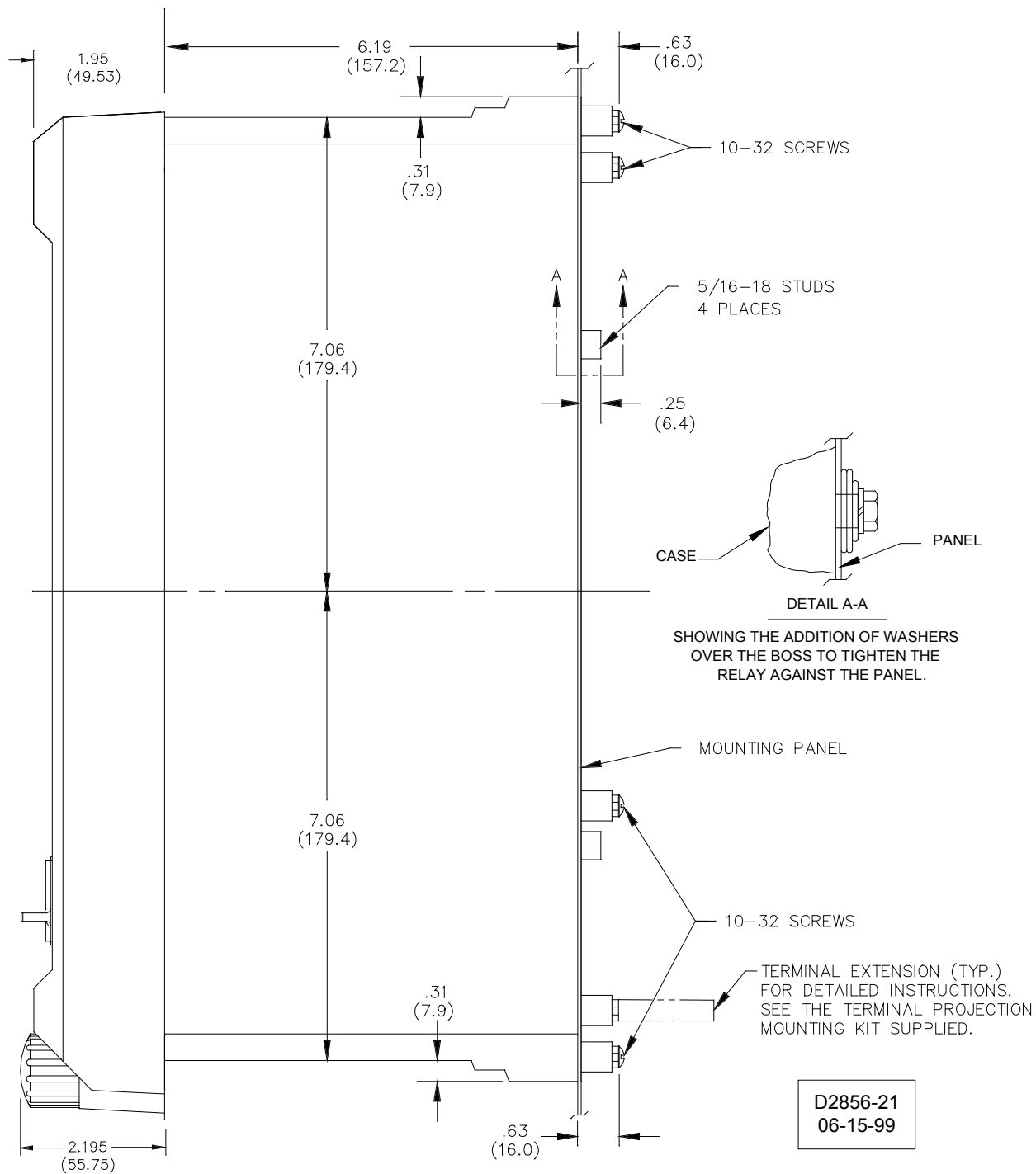
Figure 4-17. M1 Case Dimensions, Projection Mounting, Side View
