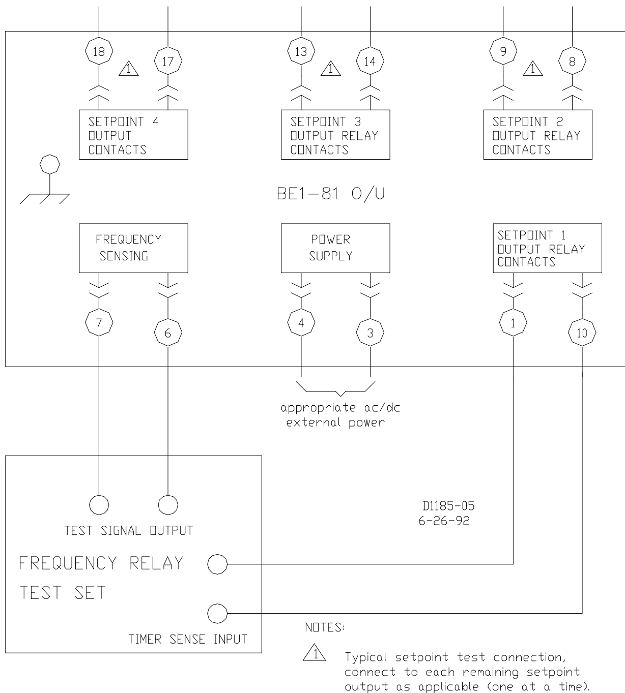
Figure 5-1. BE1-81O/U Test Setup
