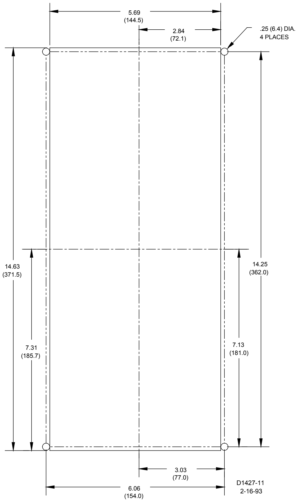
Figure 4-12. M1 Case, Panel Cutting Diagram, Semi-Flush Mounting
