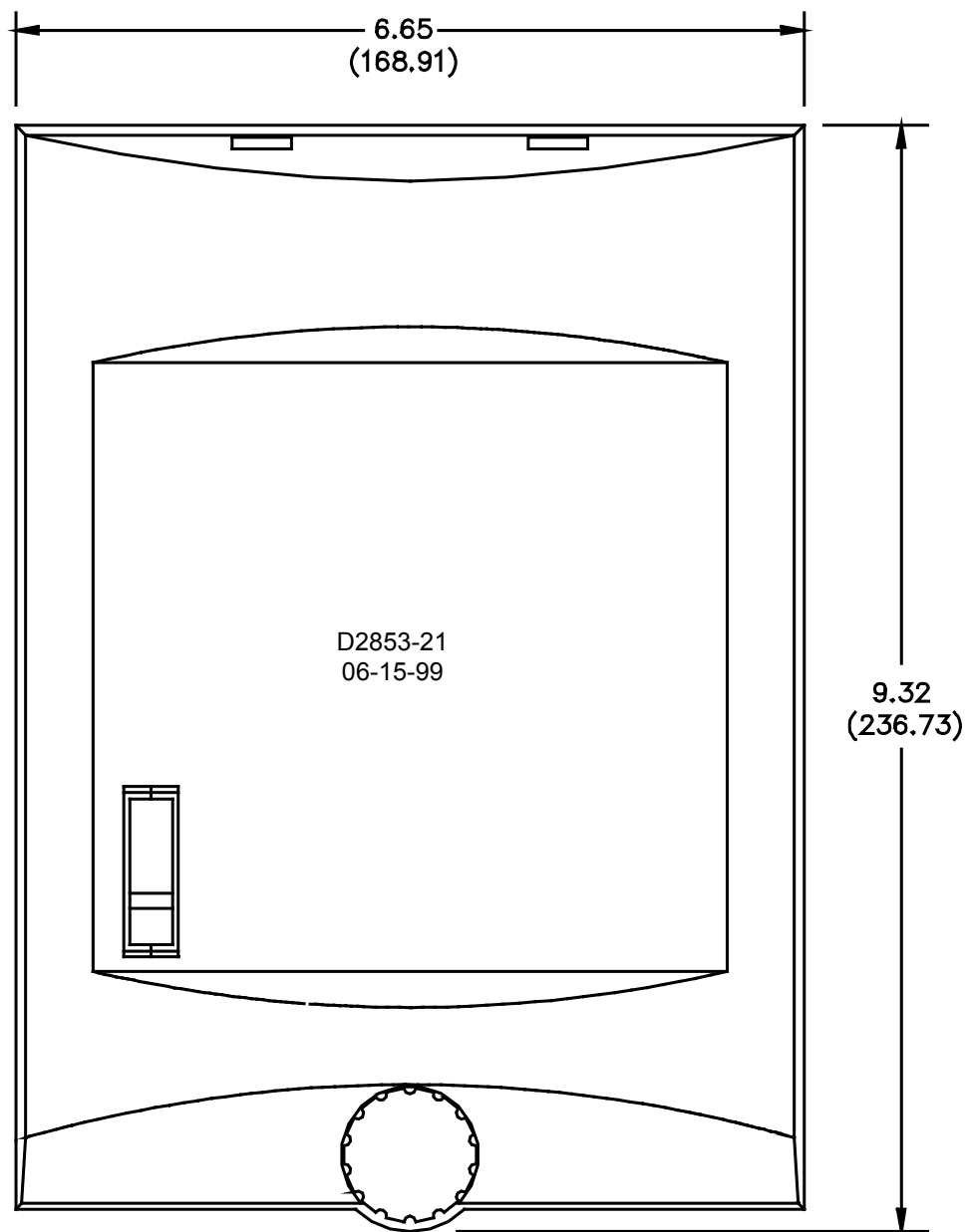
Figure 4-4. S1 Case (Cover) Dimensions, Front View
