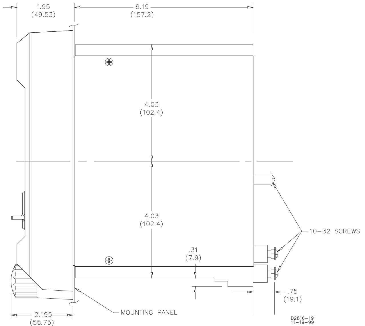
Figure 4-10. S1 Case Dimensions, Single-Ended, Semi-Flush Mounting, Side View
