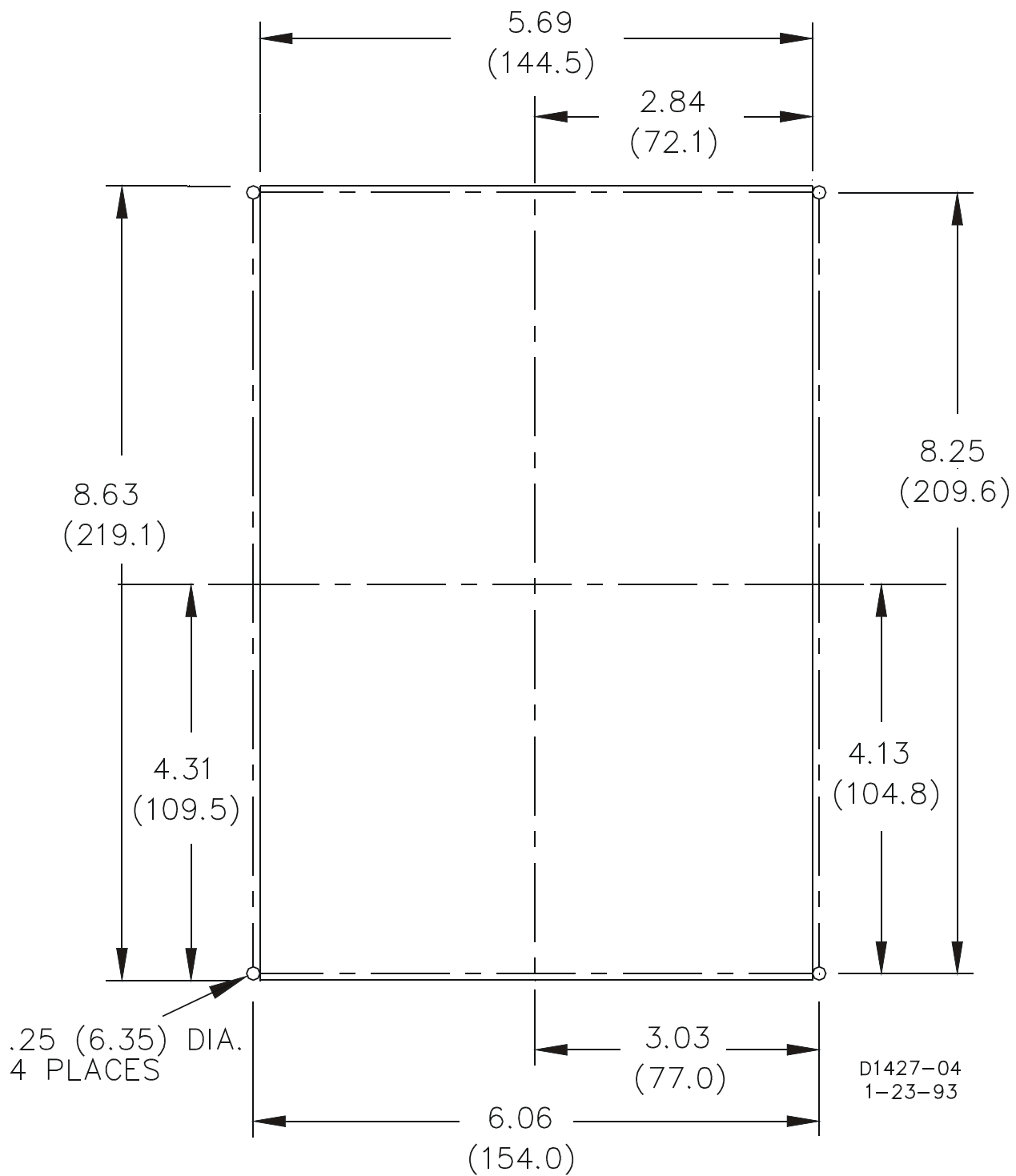
Figure 4-1. S1 Case, Panel Cutting Diagram, Semi-Flush Mounting
