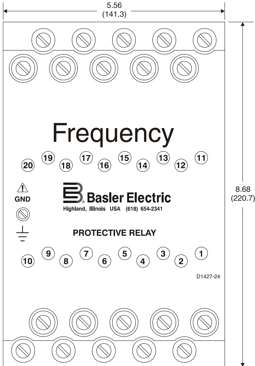
Figure 4-5. S1 Case Dimensions, Double-Ended, Rear View
