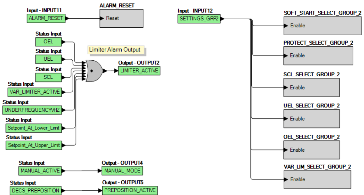
Figure 124. PSS-Disabled Default Logic - Logic Page 2 Tab
