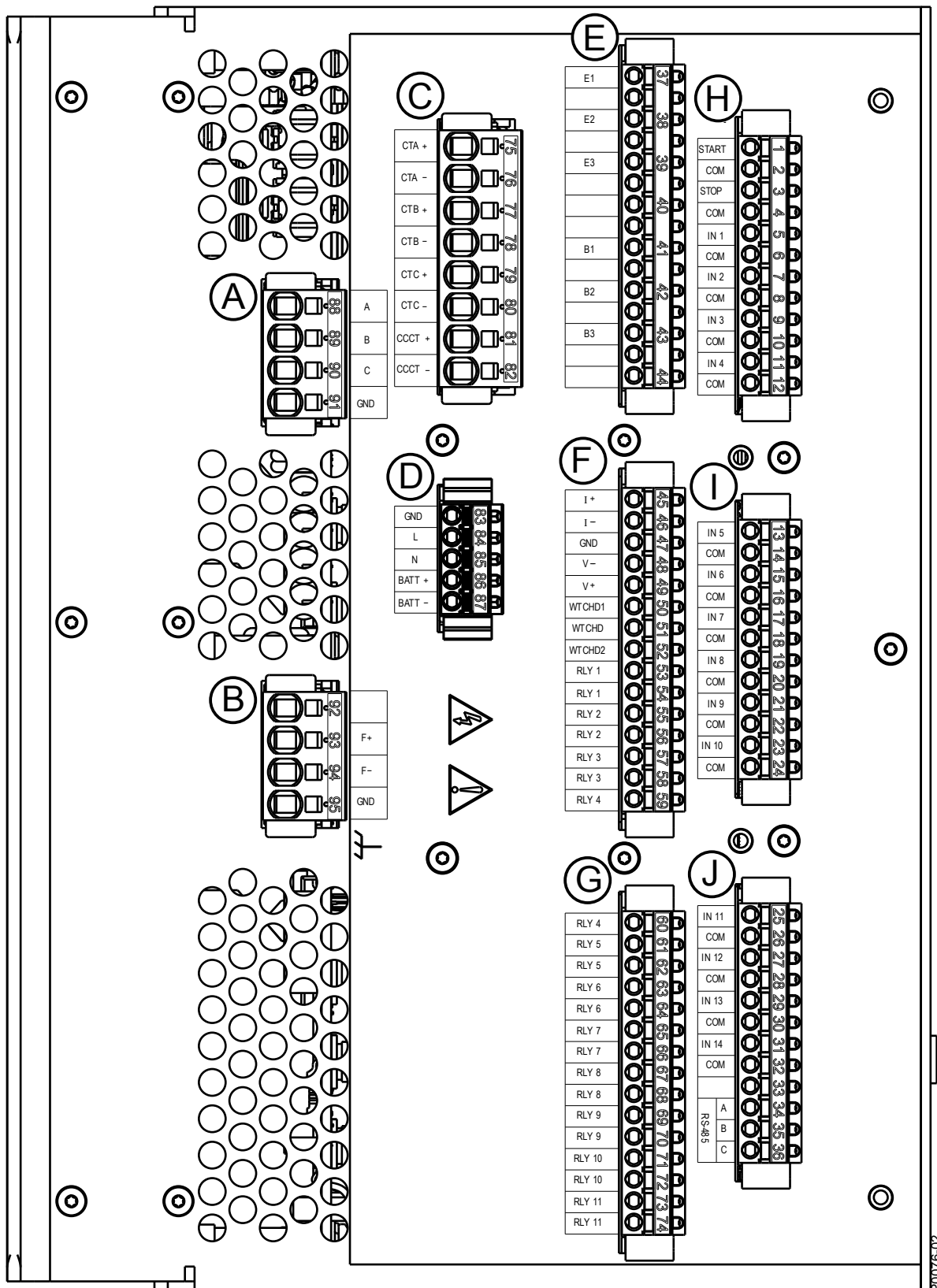
Figure 106. Left Side Panel Terminals
