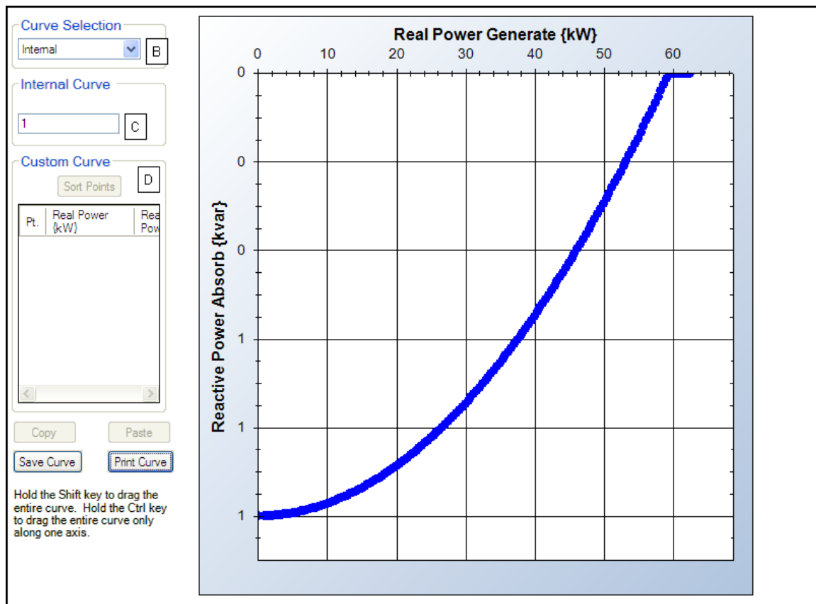
Figure 49. UEL Custom Curve Screen
