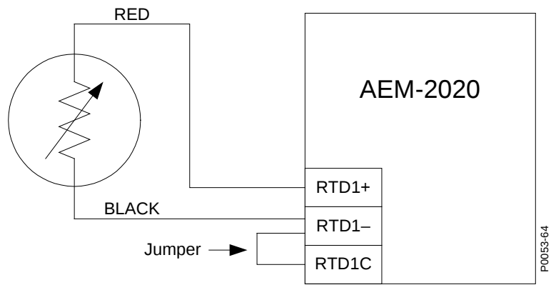
Figure 169. External Two-Wire RTD Input Connections
