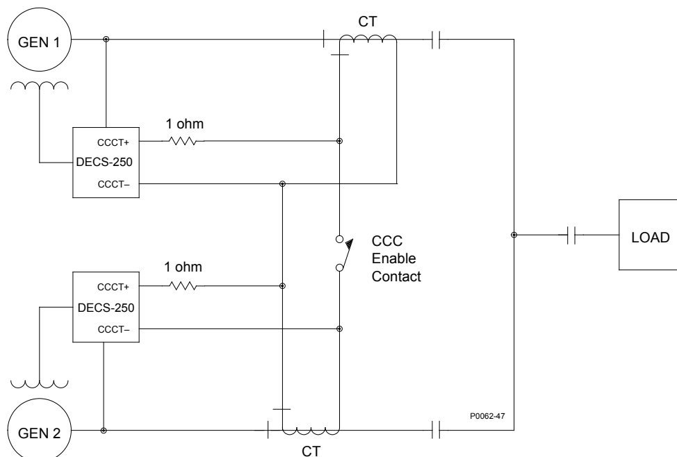
Figure 7. Connections for Cross-Current Compensation
