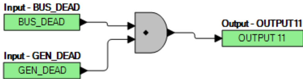
Figure 133. Example 2 - AND Gate Connections
