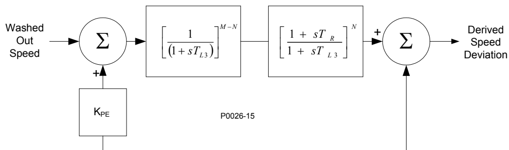
Figure 86. Derived Mechanical Power Signal
