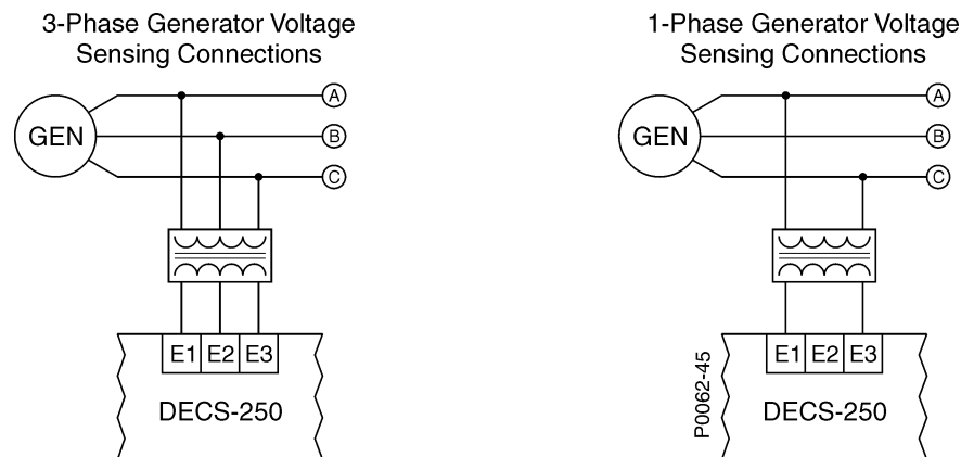
Figure 5. Typical Generator Voltage Sensing Connections
