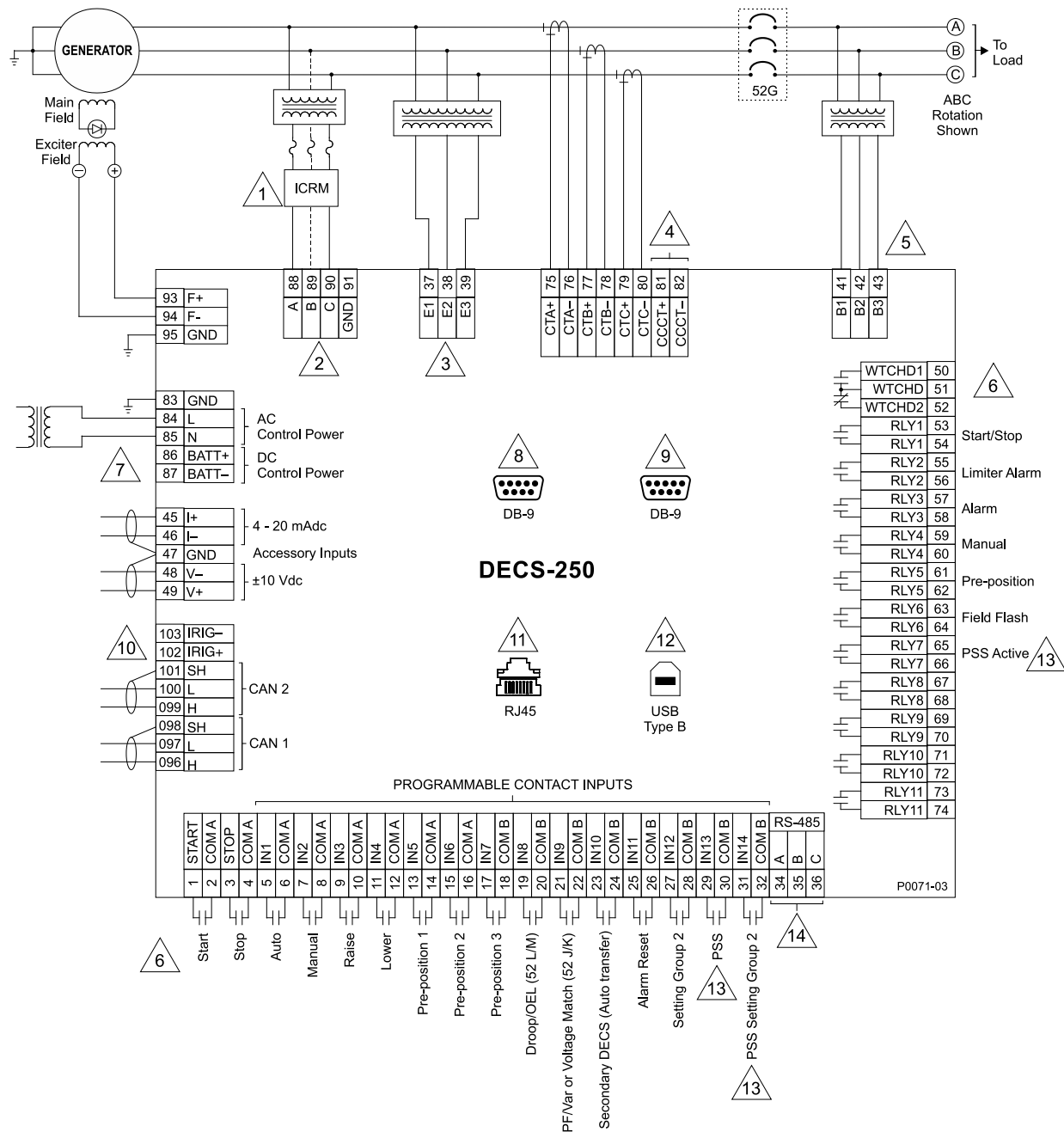
Figure 108. Typical DECS-250 Connections
