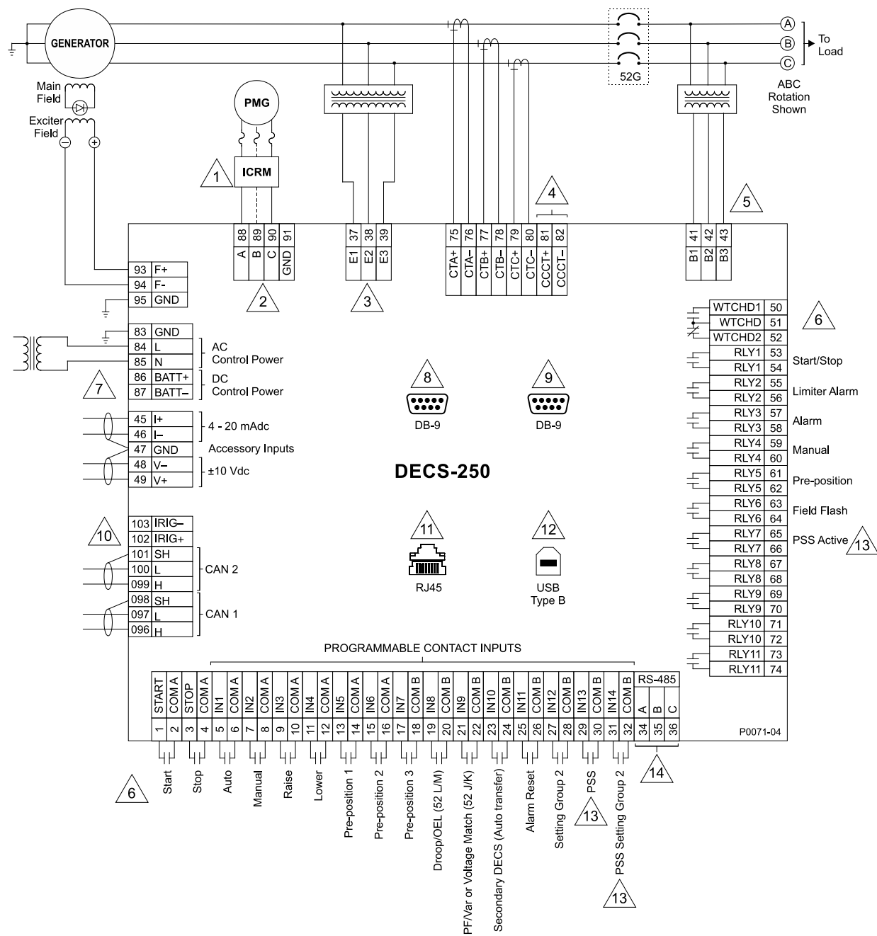
Figure 109. Typical DECS-250 PMG Connections
