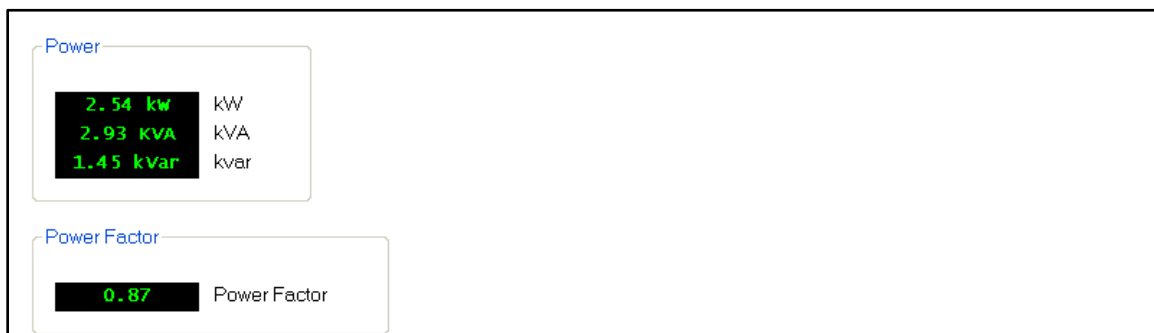
Figure 59. Power Primary-Values
