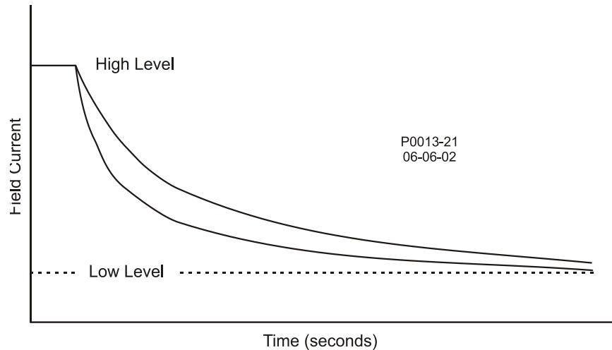
Figure 46. Inverse Time Characteristic for Takeover OEL
