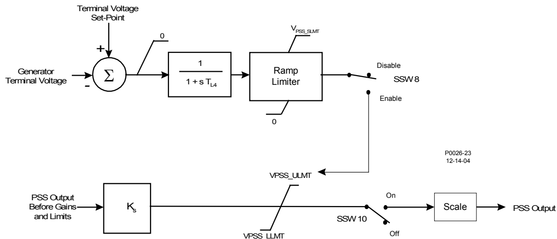
Figure 91. Output Stage
