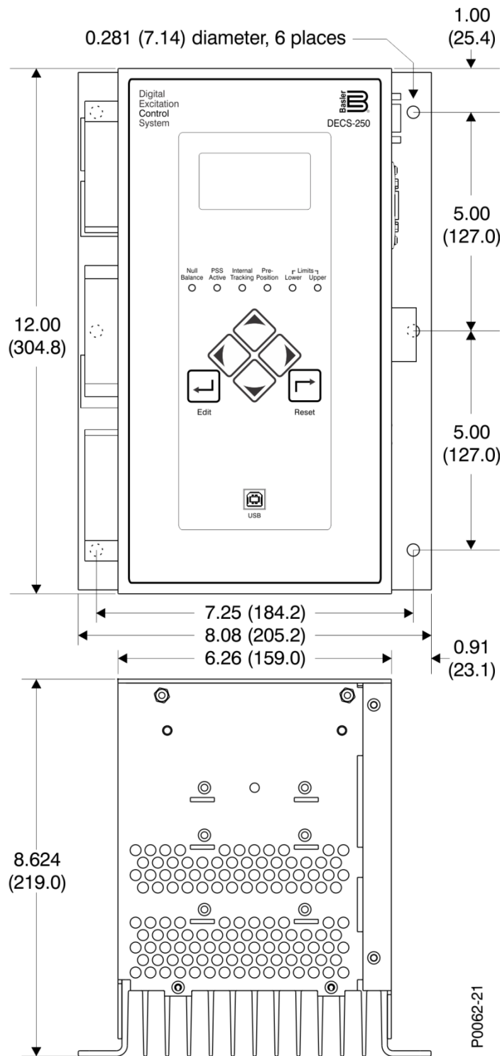
Figure 103. Overall and Projection Mounting Dimensions
