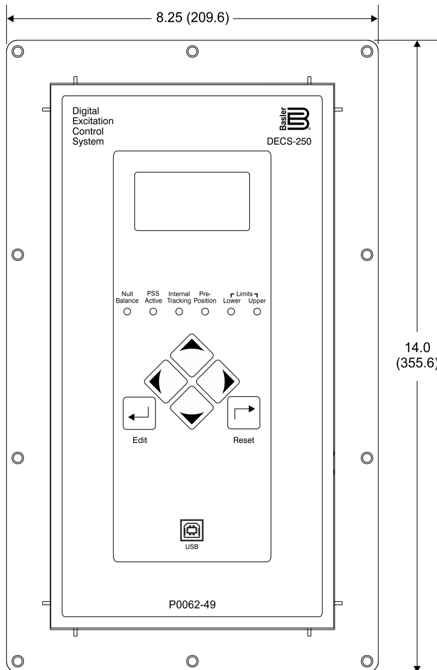
Figure 104. DECS-250 Escutcheon Plate Dimensions
