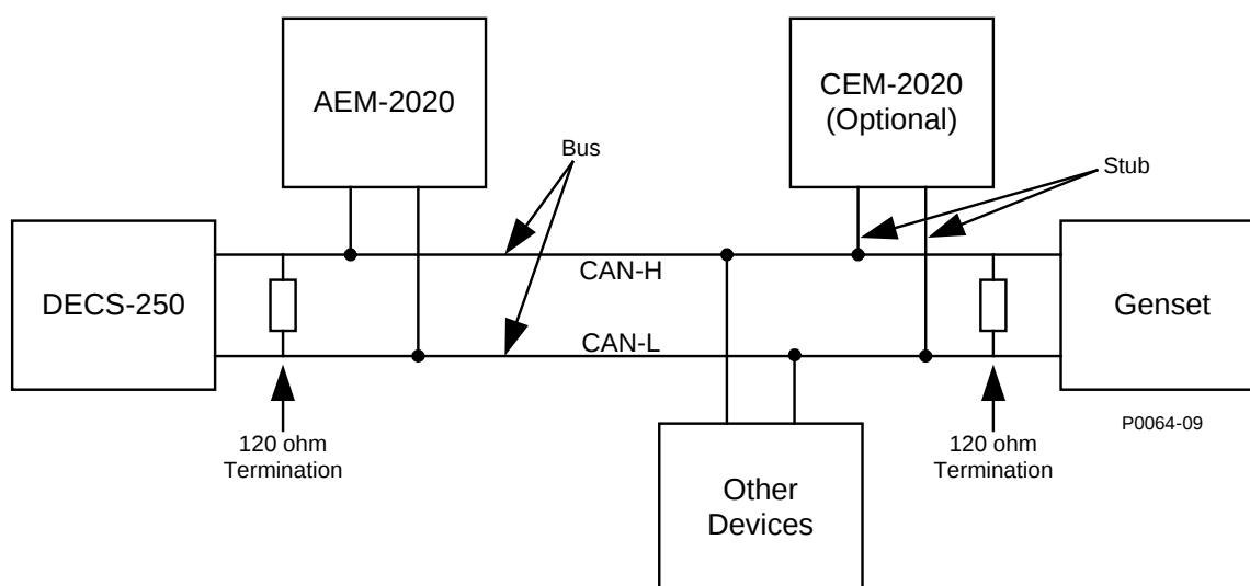
Figure 172. CAN bus Interface with DECS-250 providing One End of the Bus
