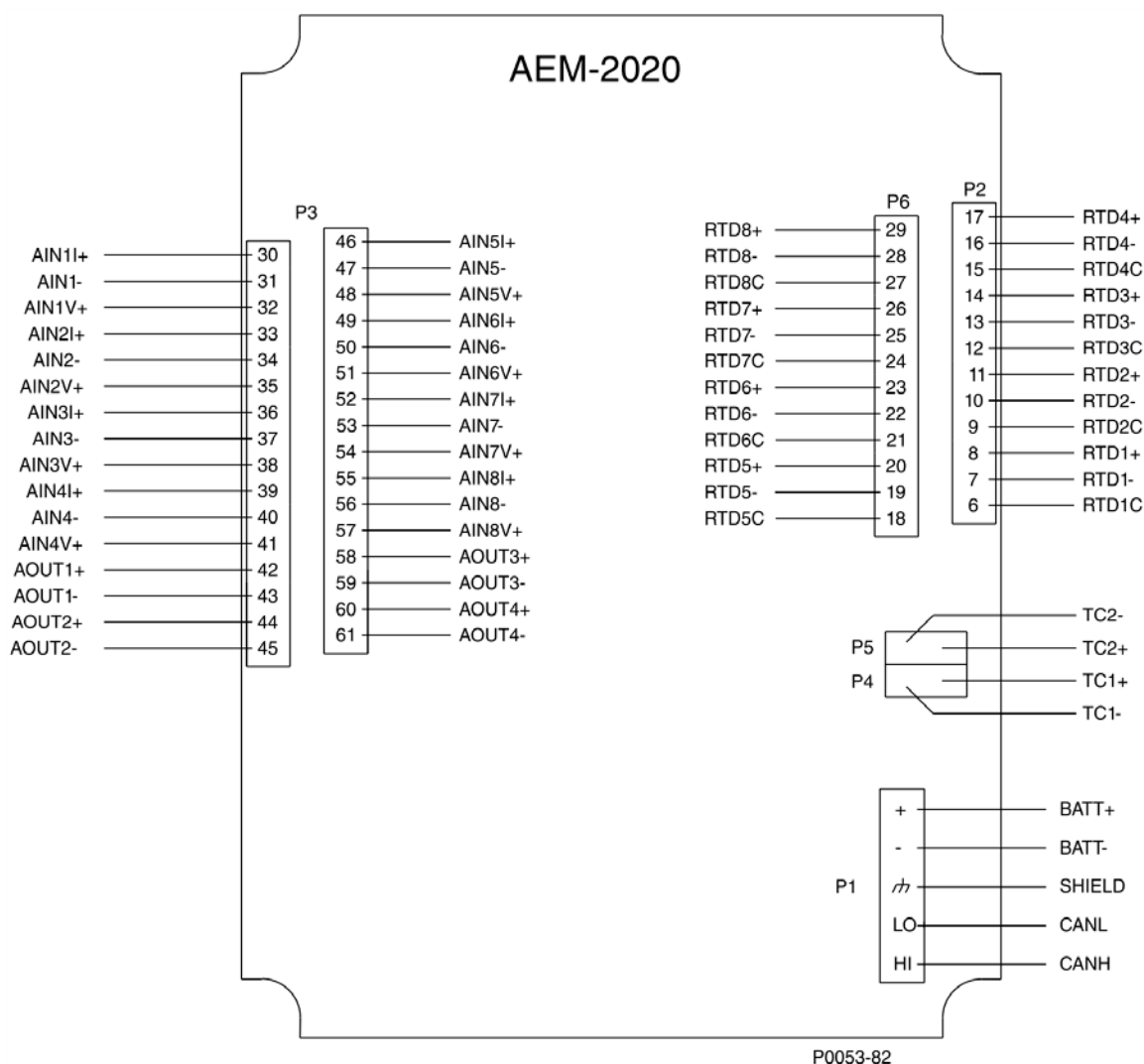
Figure 166. Input and Output Terminals
