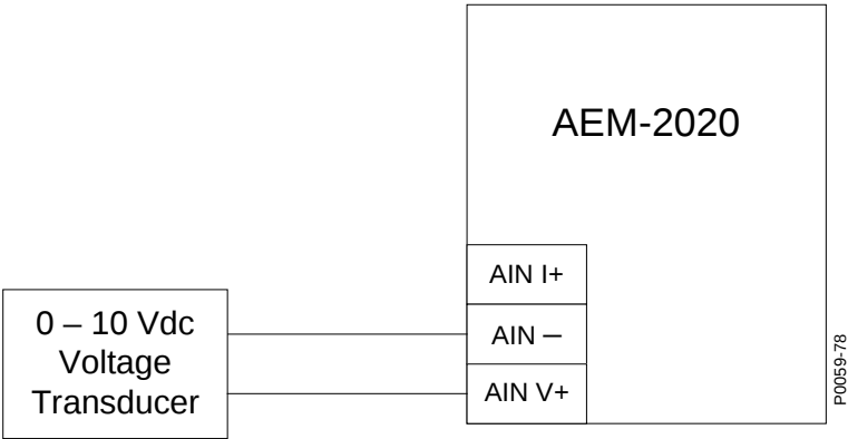
Figure 167. Analog Inputs - Voltage Input Connections
