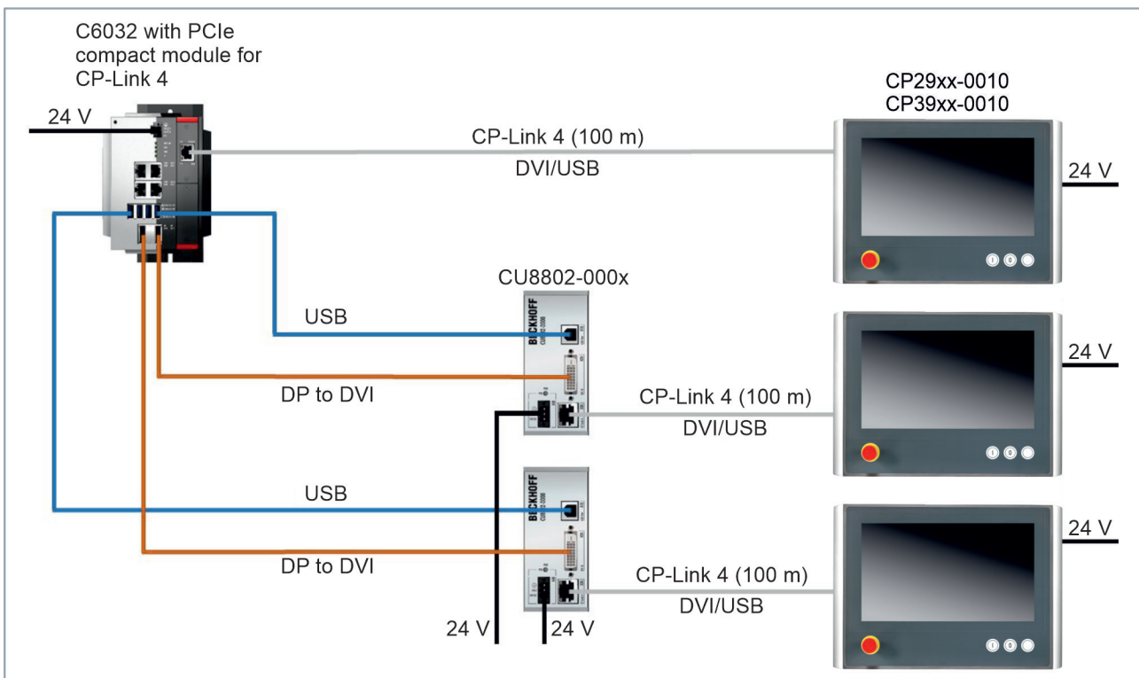
Fig. 13: CP-Link 4, CU8802
