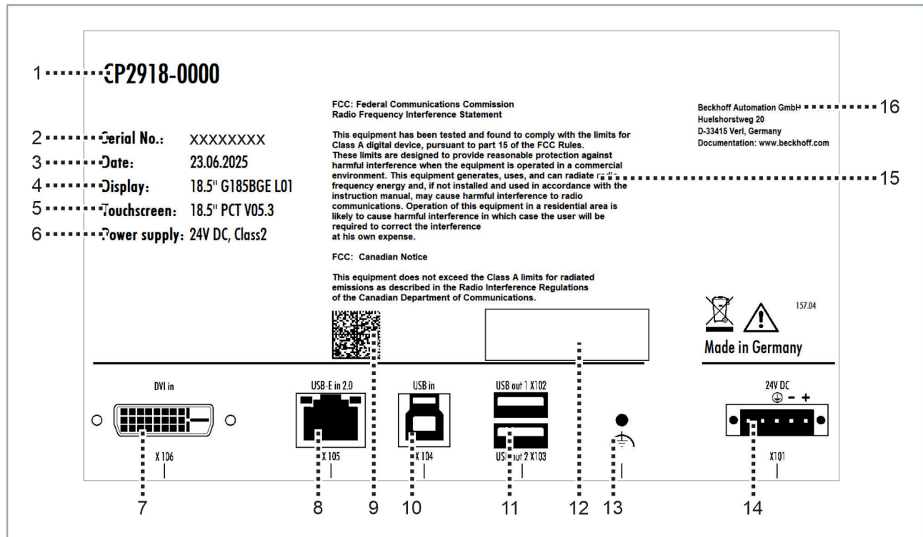
Fig. 17: Name plate example
