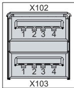
Fig. 10: USB interface pin numbering
