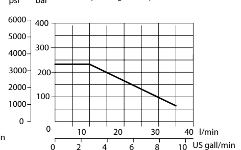
Operating envelope
