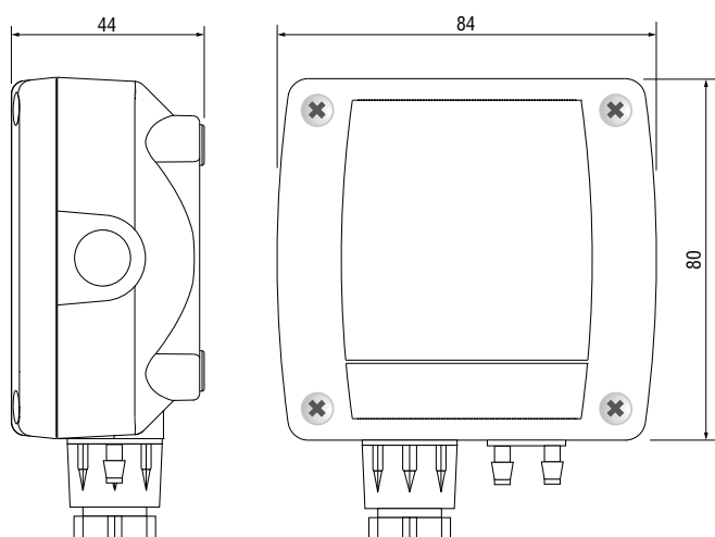
Fig. 2: dimensions (mm)
