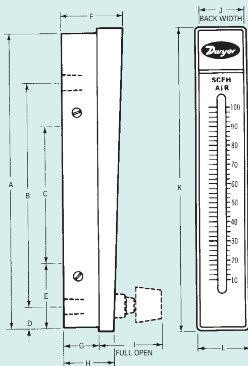
Dimension in Inches
