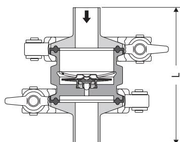
SMK 22-81, SMK 22-82 STERline®
