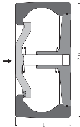
RK 41/RK 44/RK 44S DN 125 – 200 mm
