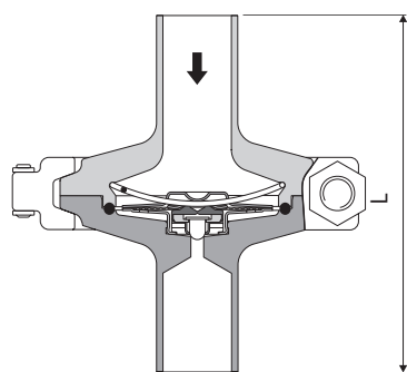
SMK 22, DN 15 STERline®
