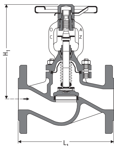
Belows-sealed stop valve GAV...F with safety stuffing box
