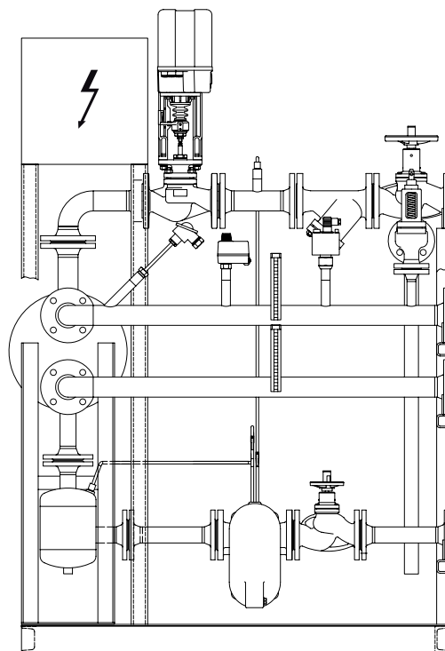
GESTRA heat exchanger unit type PWT-XPS
