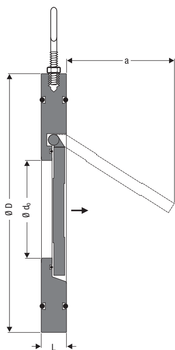
WB 26, WB 26A, WB 24 S DN 50 – 300 mm
