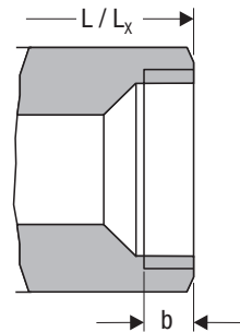
Screwed socket (UNA 26h) L x = length of installation for UNA 26h stainless steel.
