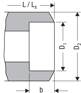
Socket-weld end (UNA 26h) L x = length of installation for UNA 26h stainless steel.
