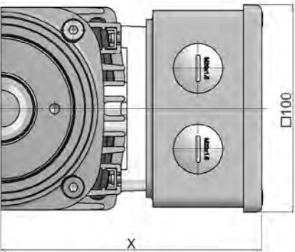
Ausführung 3: Standardausführung, x = 127 / Design 3: Standard design, x = 127
