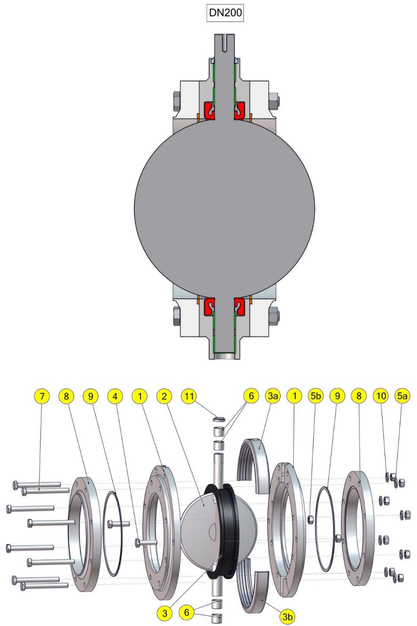
Intermediate flange-butterfly valve DN200
