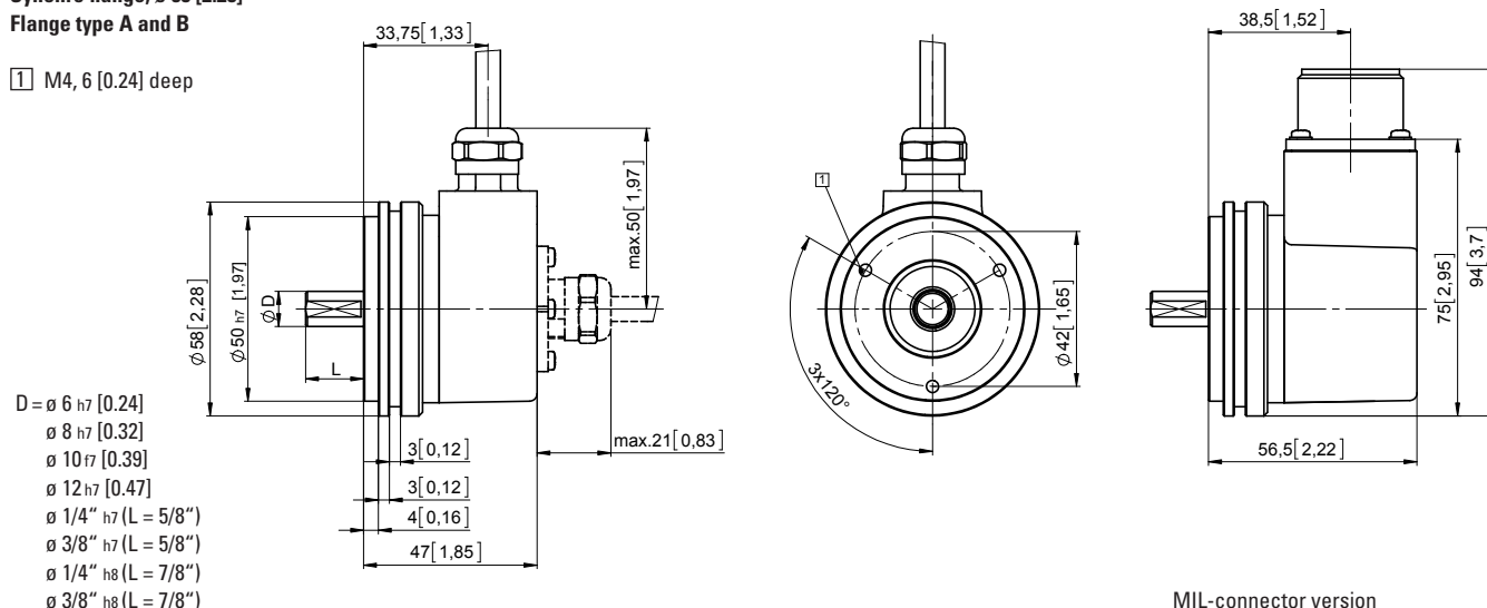
MIL-connector version
