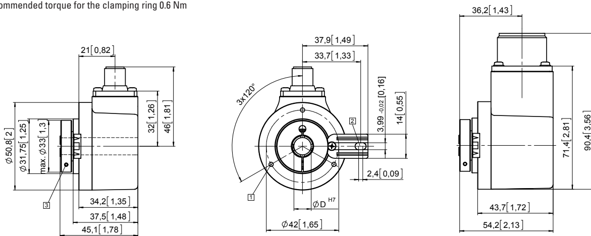
MIL-connector version
