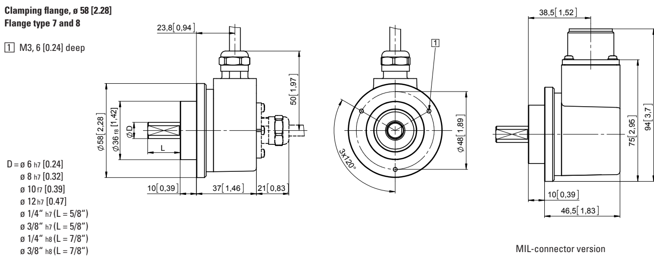
MIL-connector version
