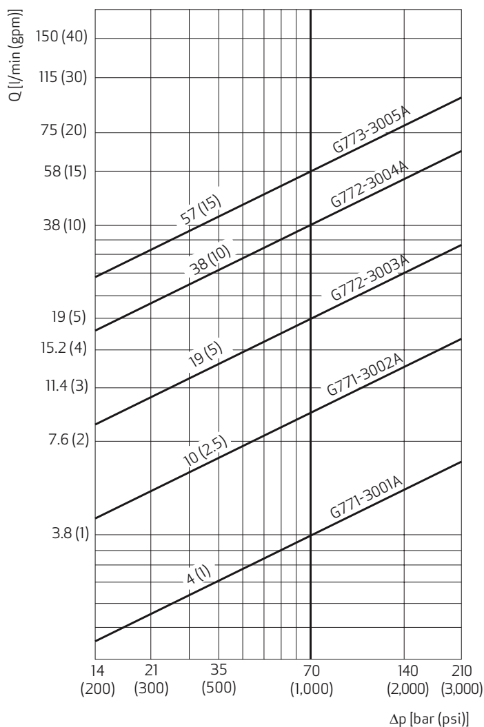
Flow Diagram
