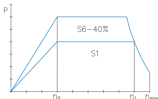
POWER DIAGRAM
