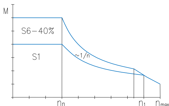
TORQUE DIAGRAM
