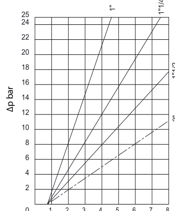
diagramma 13 diagram 13 testa head Ø50
