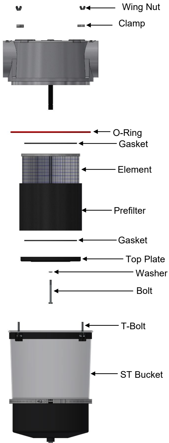
ST Series 6" "T" Style Vacuum Filter Available Replacement Parts
