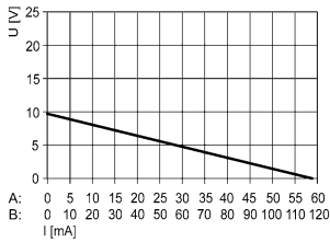
Output characteristic 9175/0-12-11, 9176/0-12-00
