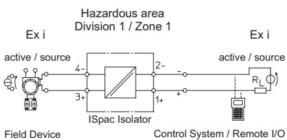
Connection Diagram 9164/13-2.-08
