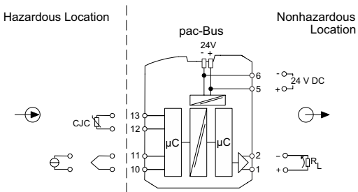
Connection diagram 9282/12-51-16
