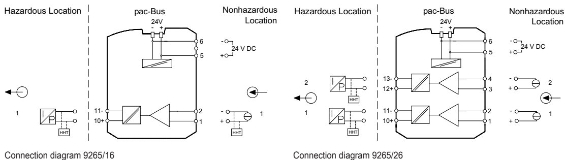
Connection diagram 9265/16
