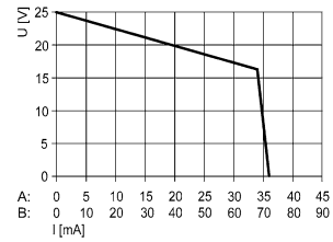
Output characteristic 9175/0-16-11; 9176/0-16-00
