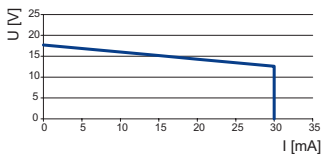
Output characteristic 9475/33-08-50
