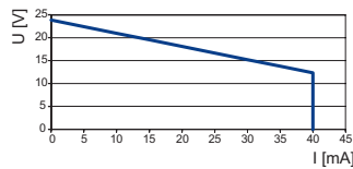
Output characteristic 9475/32-04-22
