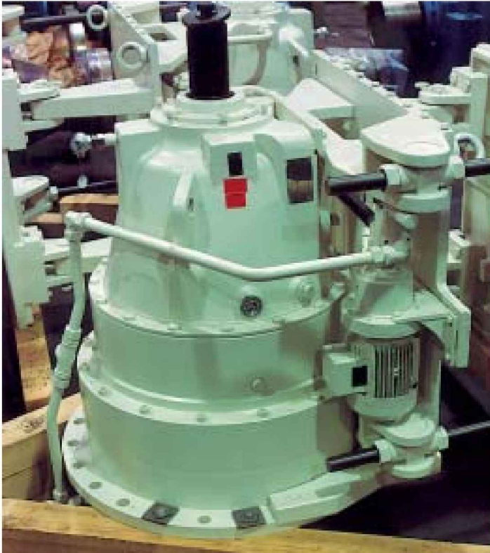
Gear pump SF for gear-unit lubrication
