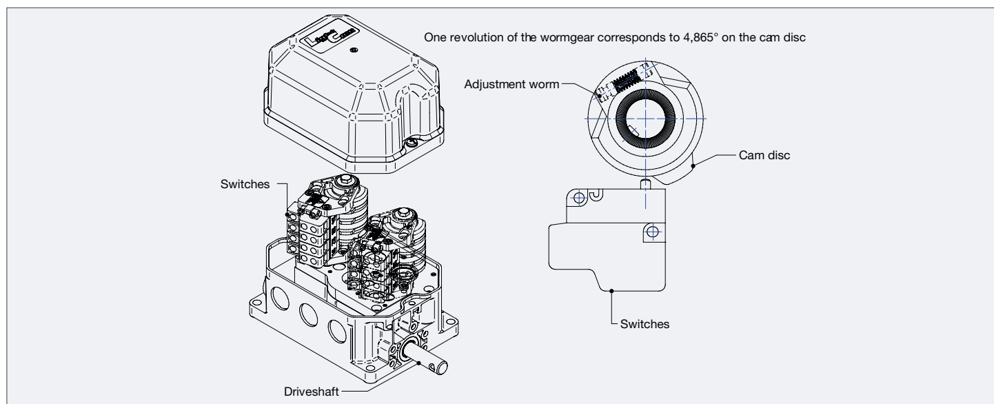
Gear table, for switches 99, 99A, 99G, 99T, 99P with cam discs 40° FV
