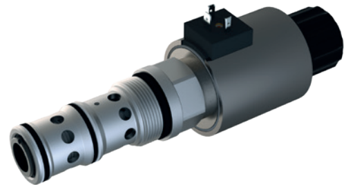
Cartridge execution
