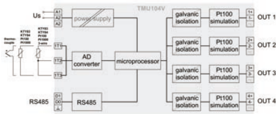
Block diagram
