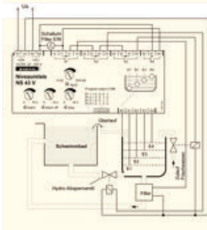
Program 6 Pool control for overflow bassin with switching of hydro-lock valve, dosing of fresh water, emergency filter-on and protection from running dry.
