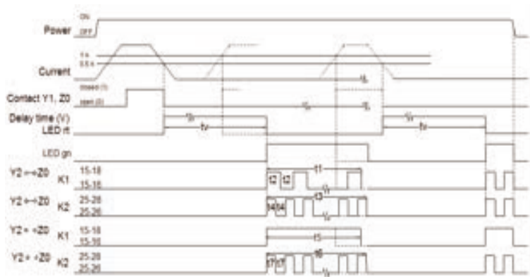
Function diagram:
