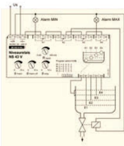
Program 1 Control of dose or drain with 2 electrodes with 2 more electrodes to protect from overflow and running dry. The level swings between the 2 middle electrodes. Standard-program for levelling a liquid in a container.
